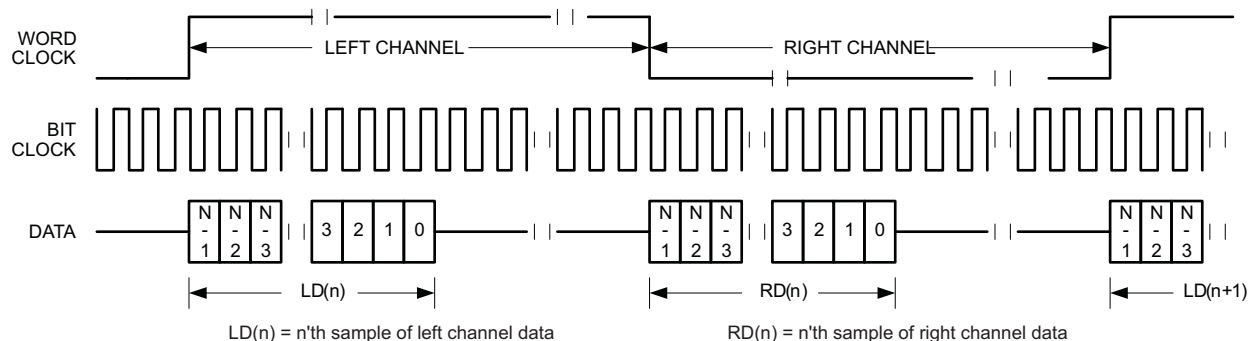
FIG 36. Timing Diagram for Left-Justified Mode
