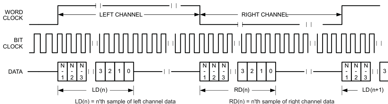
FIG 38. Timing Diagram for Left-Justified Mode with ASI_OFFSET1 = 0 and Inverted Bit Clock
