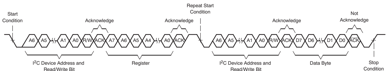
FIG 22. Single-Byte Read Transfer
