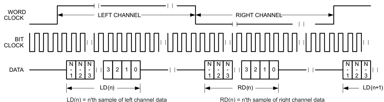
FIG 37. Timing Diagram for Left-Left Mode with ASI_OFFSET1 = 1
