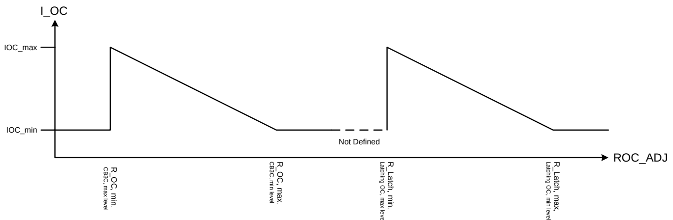
FIG 23. OC Threshold versus OC_ADJ Resistor Value Example
