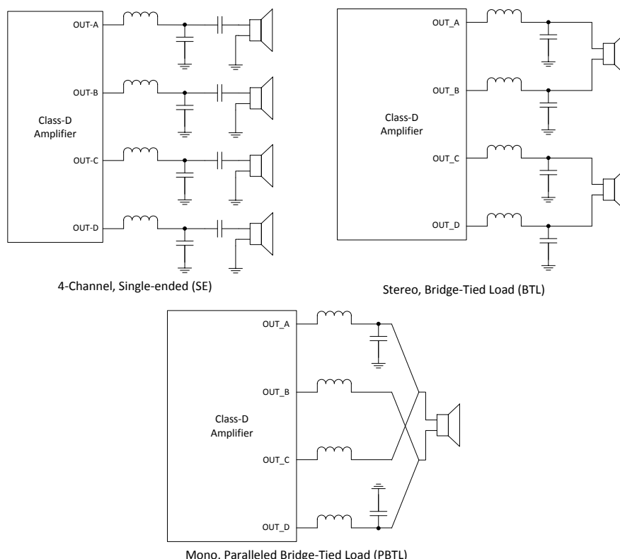
FIG 24. Device Functional Modes Configurations
