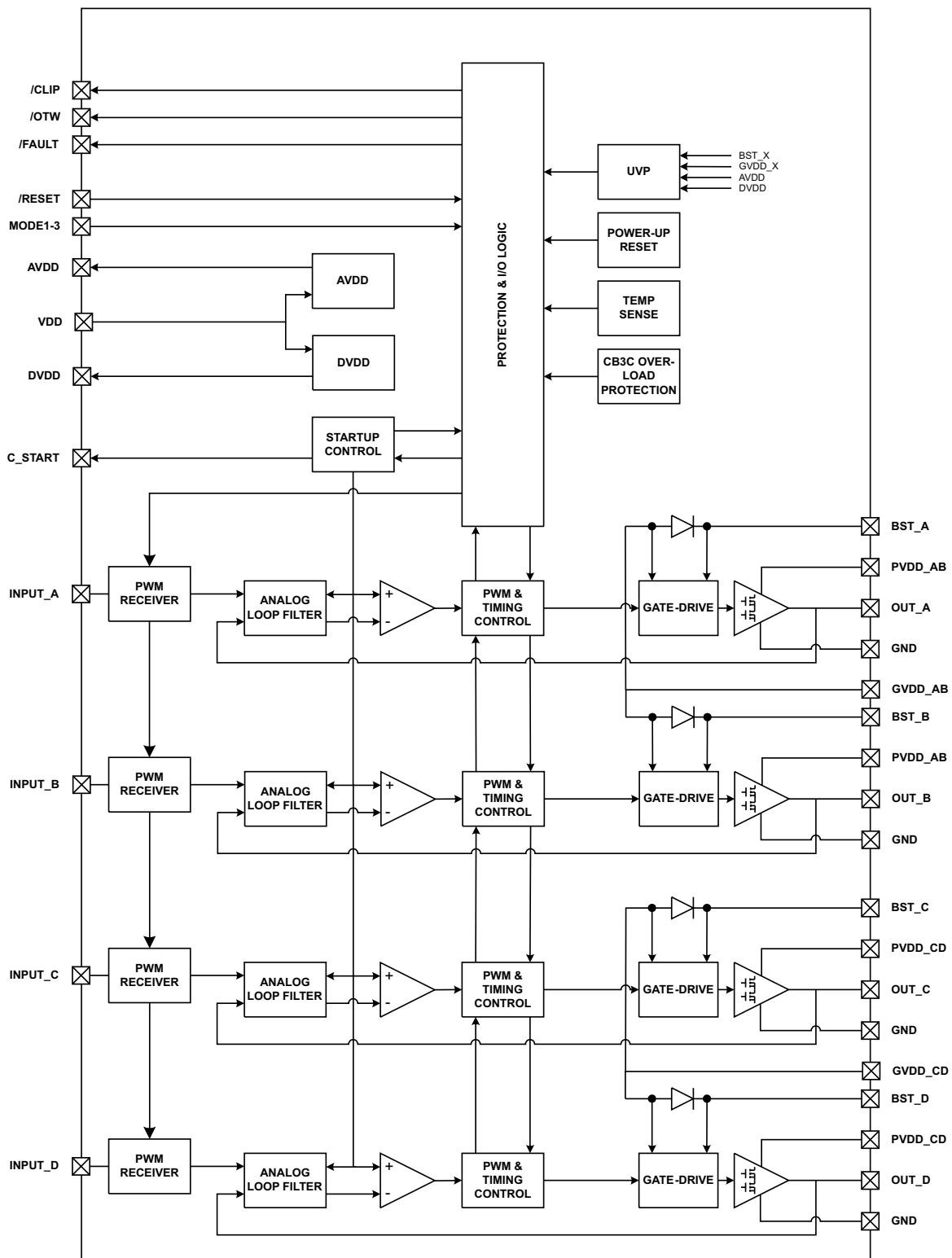
FIG 20. Functional Block Diagram
