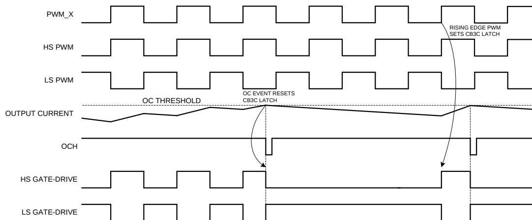
FIG 22. CB3C Timing Example
