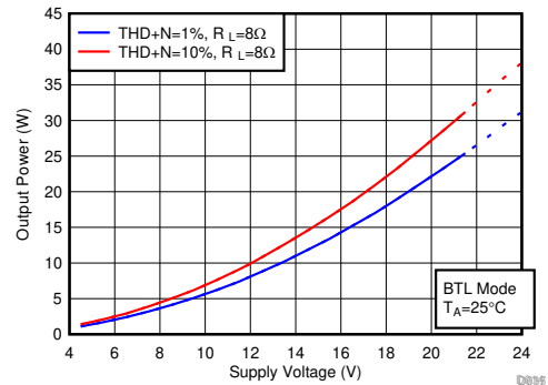
6-48. Output Power vs Supply Voltage
