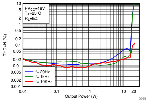
6-21. THD+N vs Output Power-BTL
