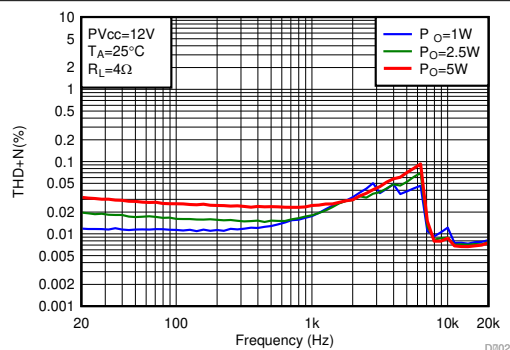
Figure 6-79. THD+N vs Frequency
