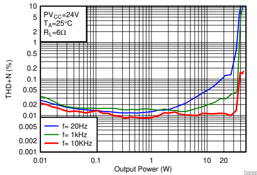
6-19. THD+N vs Output Power-BTL
