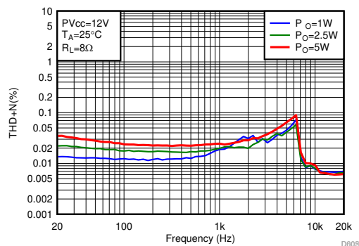
Figure 6-38. THD+N vs Frequency
