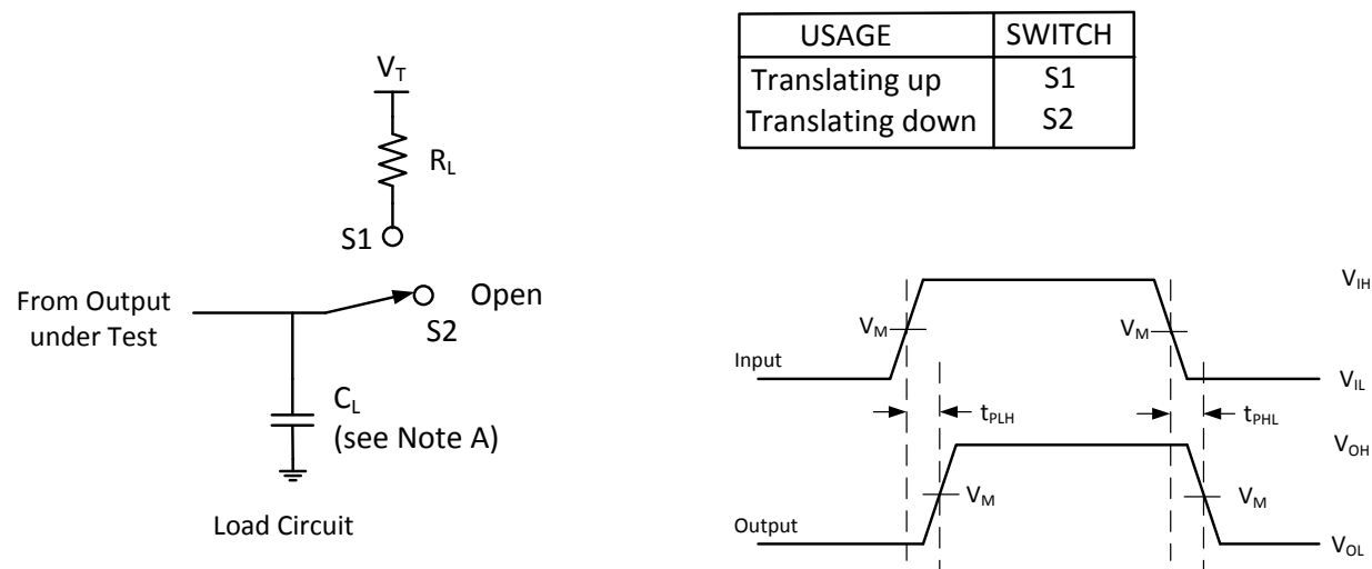
7-3. Application Setup for Propagation Delays Delay
