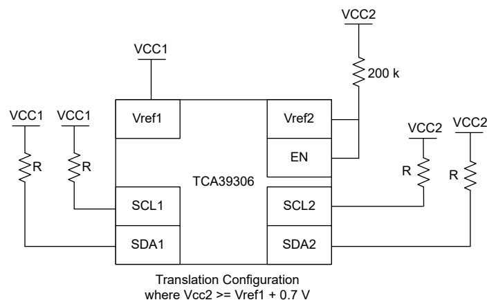
8-6. Translation Configuration
