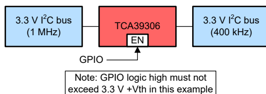
8-3. Example of an I2C bus with multiple supported frequencies
