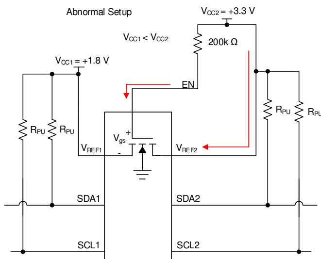
8-2. Abnormal Setup
