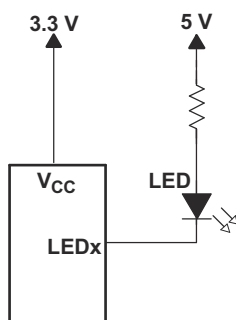
FIG 9-3. Device Supplied by a Lower Voltage
