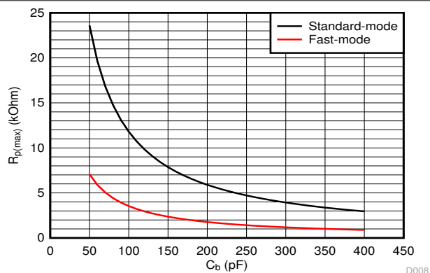
FIG 9-4. Maximum Pullup Resistance ( R_{p(max)} ) vs Bus Capacitance ( C_b )
