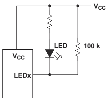
FIG 9-2. High-Value Resistor in Parallel With LED
