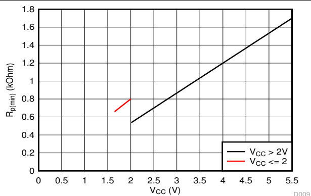
FIG 9-5. Minimum Pullup Resistance ( R_{p(min)} ) vs Pullup Reference Voltage ( V_{CC} )
