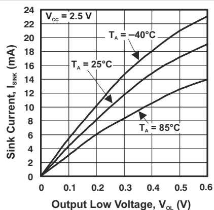
FIG 6-5. I/O Sink Current vs Output Low Voltage
