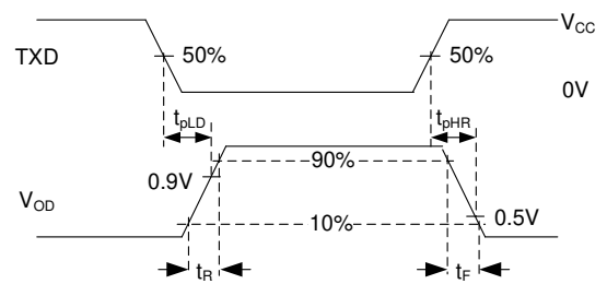
8-1. Driver Test Circuit and Measurement
