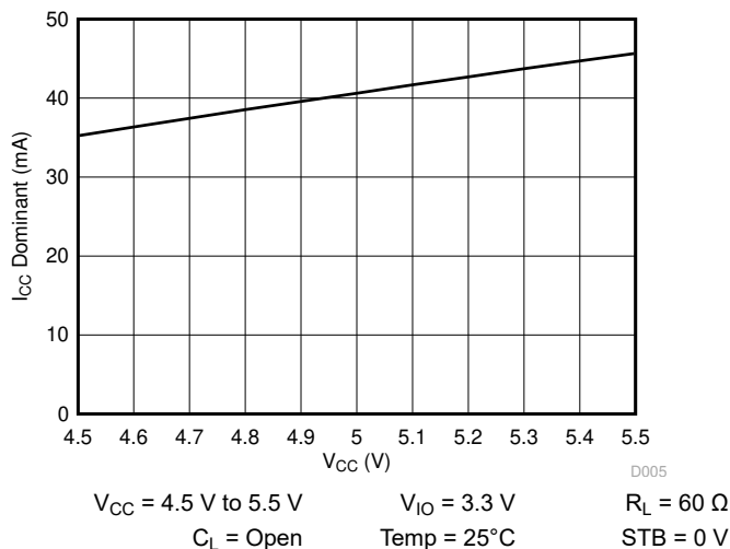
FIG 10-5. I_{CC} Dominant Current over V_{CC} Supply Voltage
