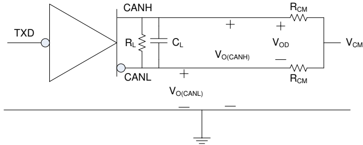
8-1. Driver Test Circuit and Measurement
