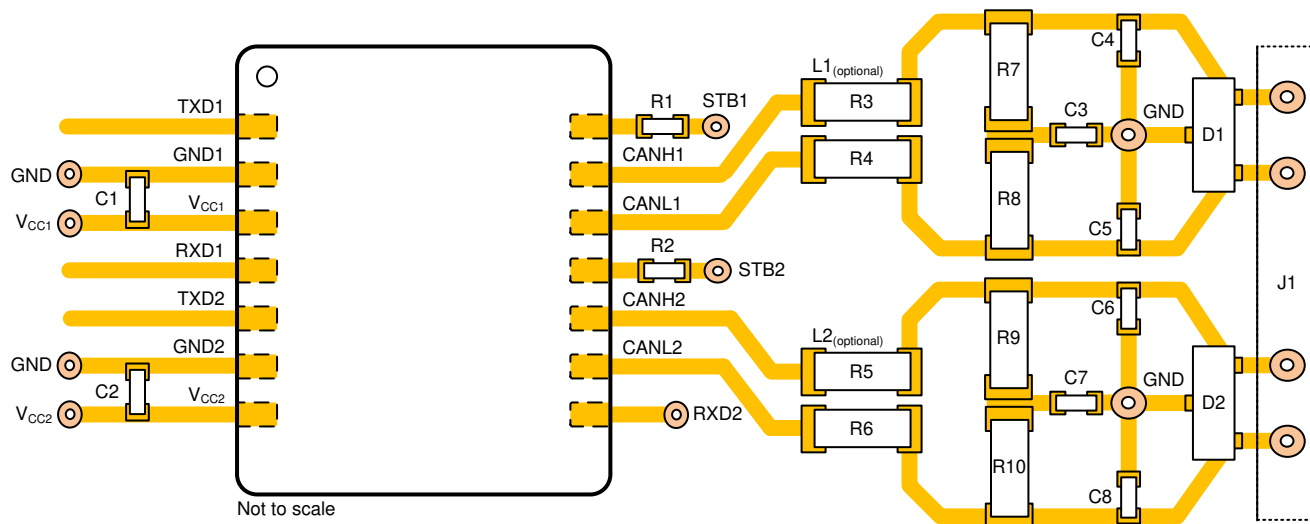
11-1. Layout Example
