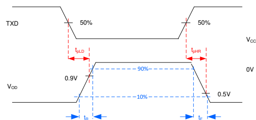
7-2. Driver Test Circuit and Measurement
