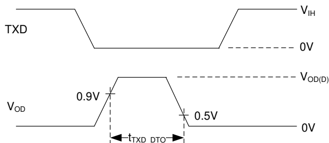
FIG 7-5. CAN FD Timing Parameter Measurement
