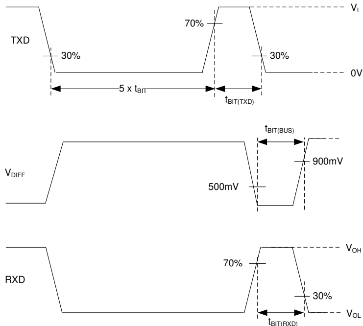
FIG 7-5. CAN FD Timing Parameter Measurement
