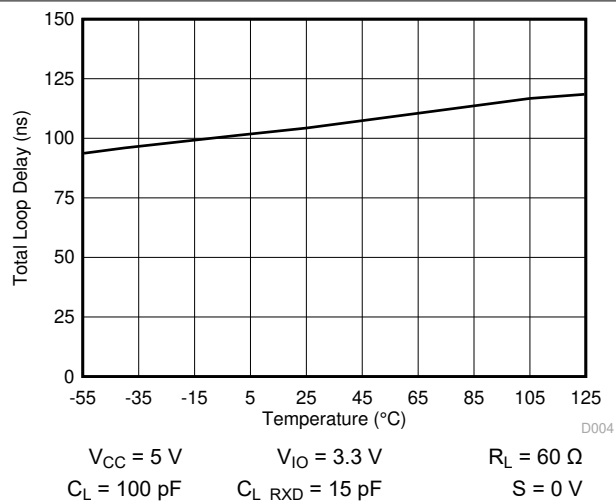
6-4. Total Loop Delay over Temperature
