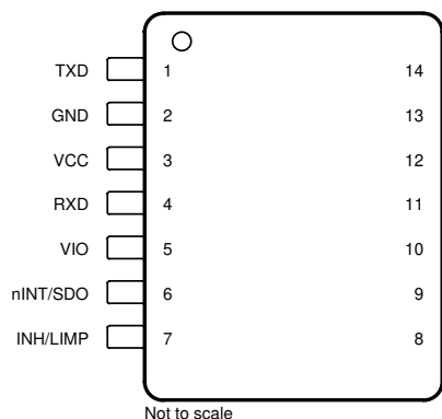
图 7-1. D Package, 14 Pin (SOIC), Top View
