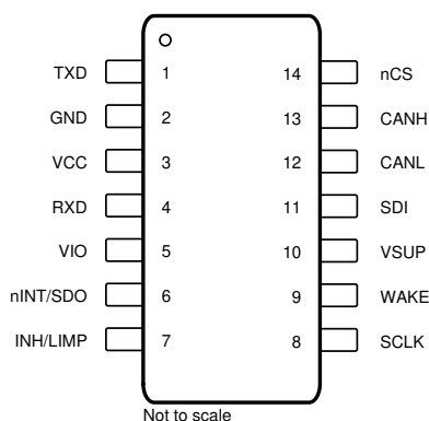
图 7-3. DYY Package, 14 Pin (SOT-23), Top View
