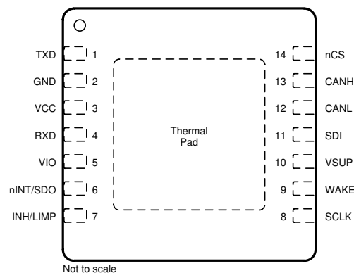
图 7-2. DMT Package, 14 Pin (VSON), Top View
