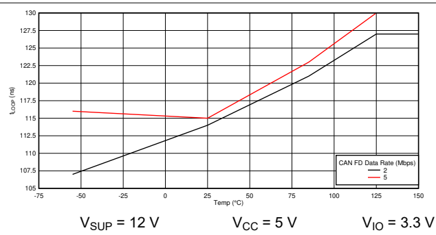
8-3. t_{LOOP} vs Temperature
