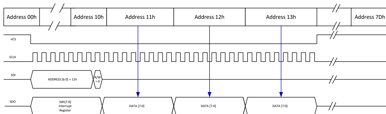
图 10-39. 32-bit SPI Burst Read
