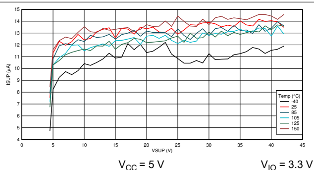
8-4. Sleep Mode: I_{SUP} vs Temperature
