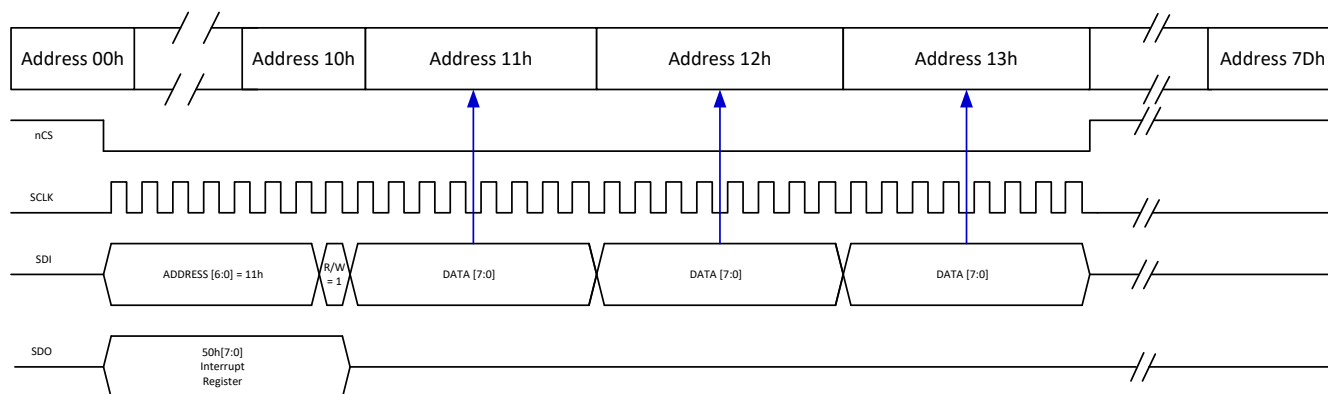
FIG 10-37. 32-bit SPI Burst Write
