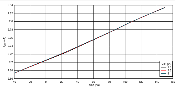
11-8. Normal Mode: I_{CC} vs Temperature Recessive
