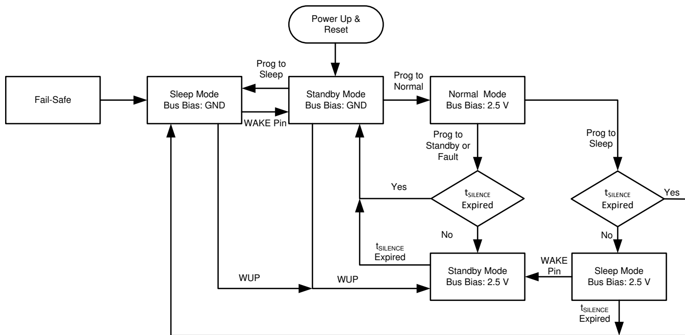
FIG 105. Bus Biasing Based on Modes of Operation
