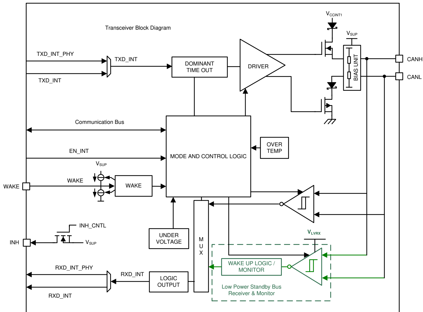
✎ 19. CAN Transceiver Block Diagram
