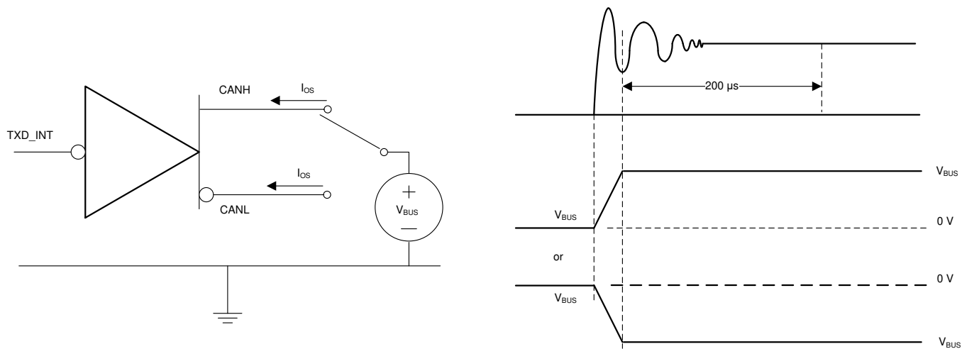
FIG 10. Driver Short-Circuit Current Test and Measurement
