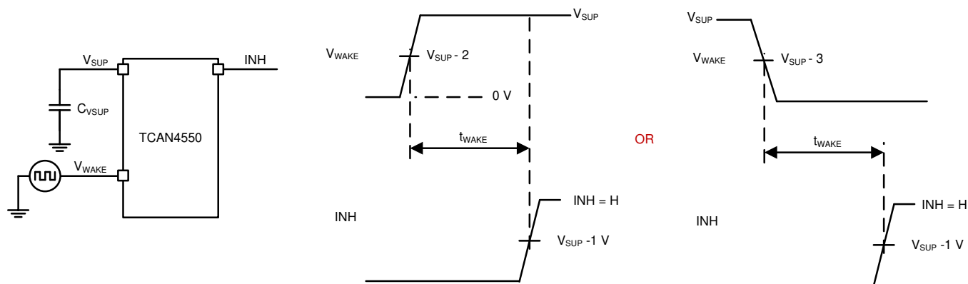
FIG 11. t_{WAKE} While Monitoring INH Output
