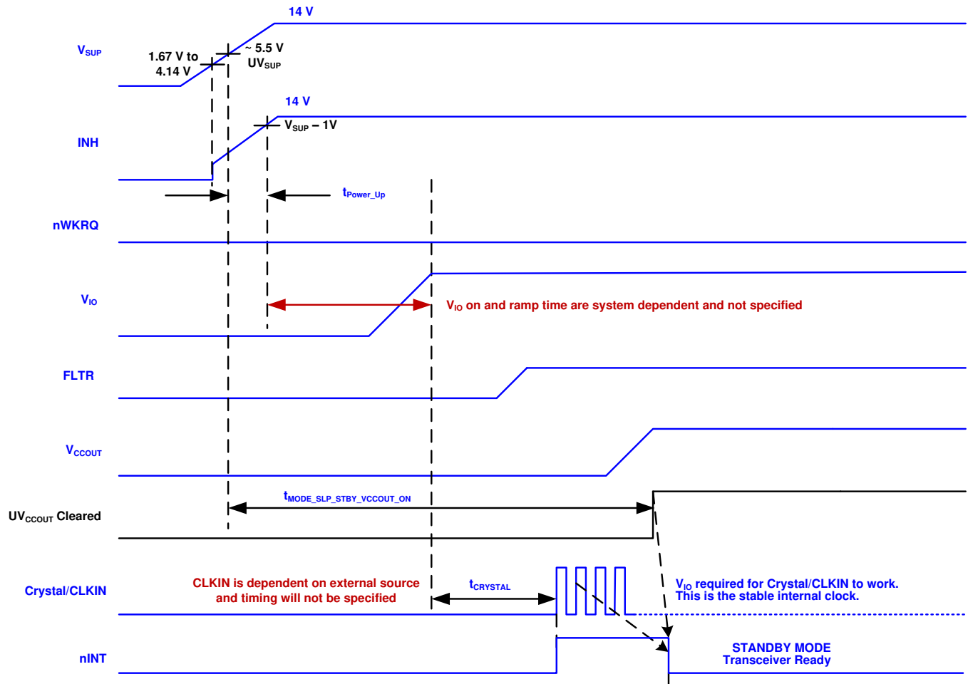
✎ 15. Power Up Timing
