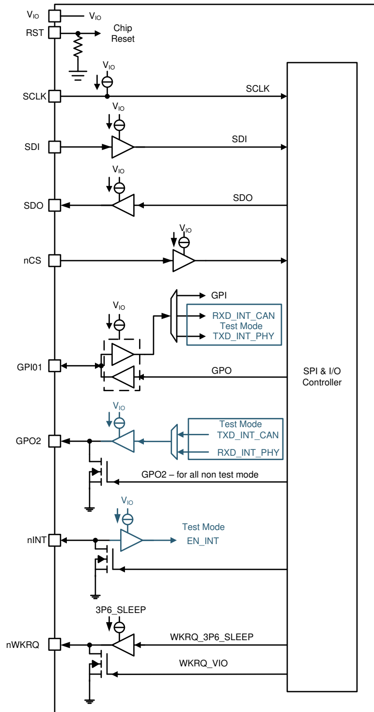
✎ 20. SPI and Digital IO Block Diagram
