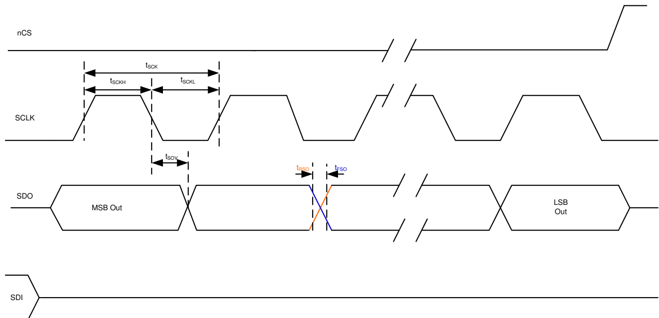
✎ 14. SPI AC Characteristic Read
