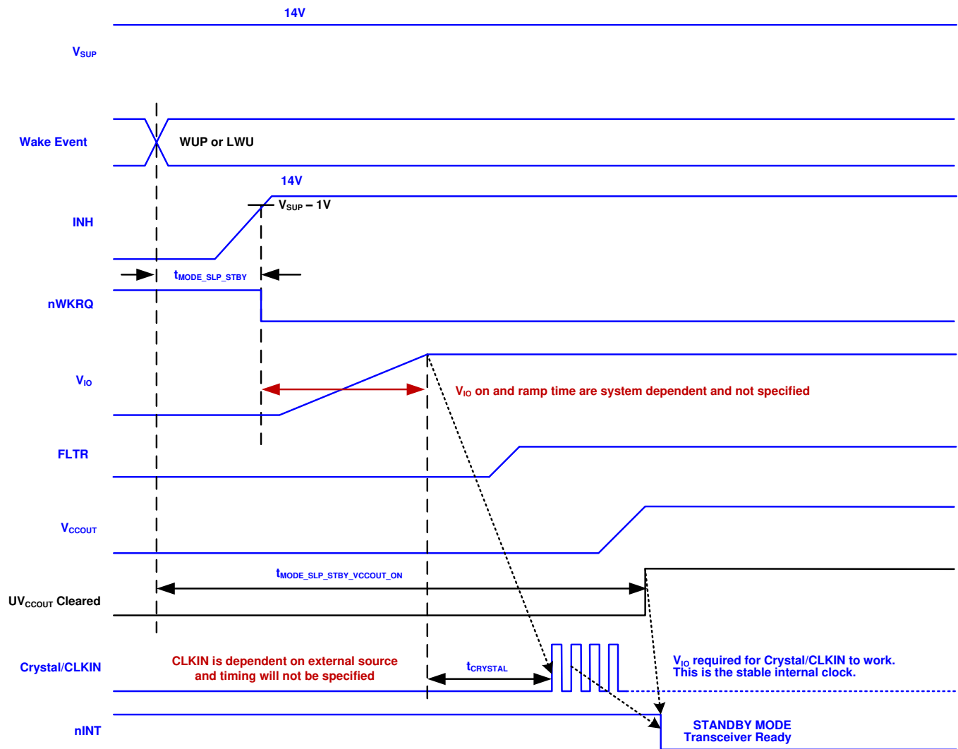
16. Sleep to Standby Timing
