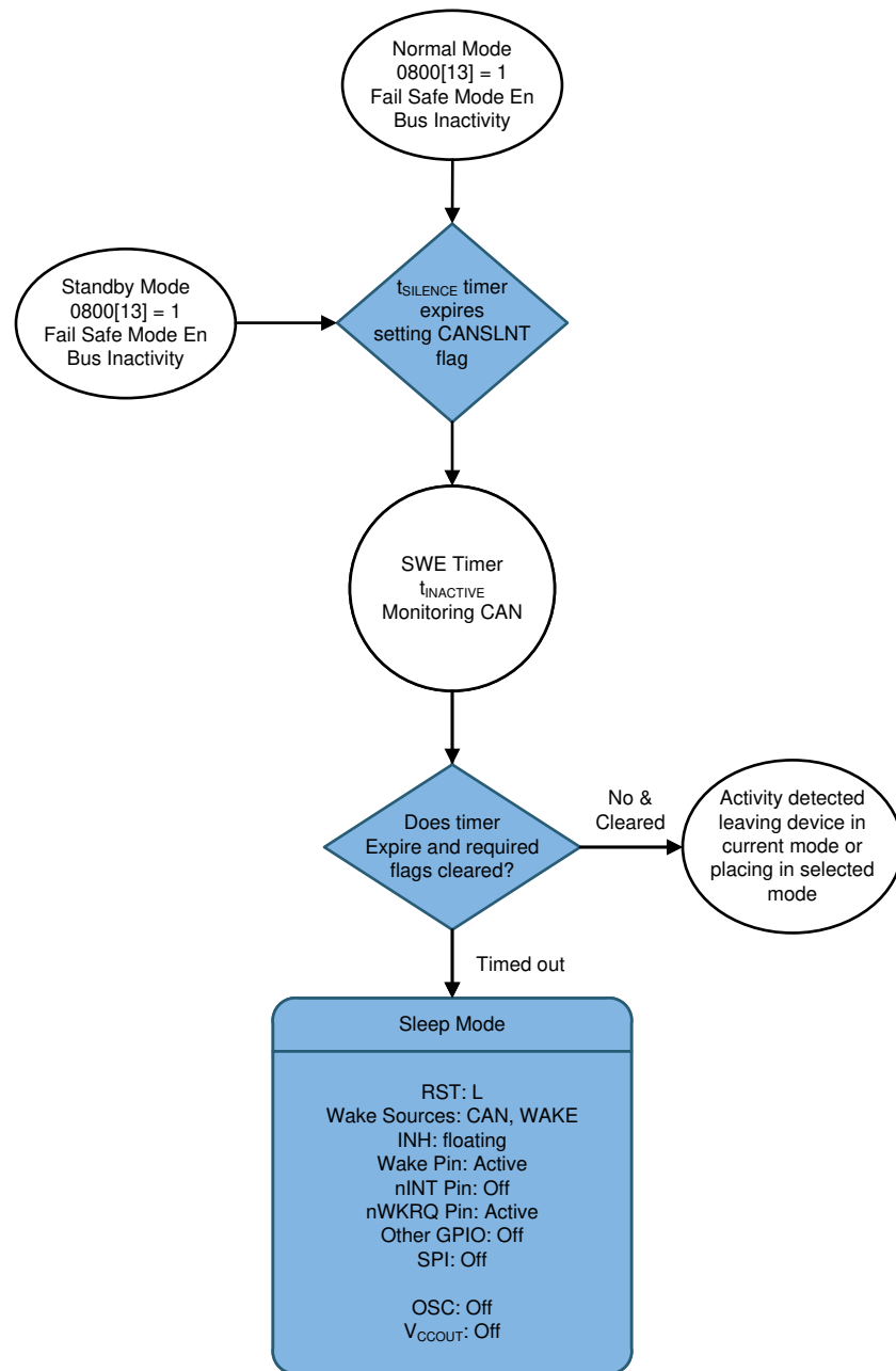
✉ 33. Normal and Standby Failsafe Feature
