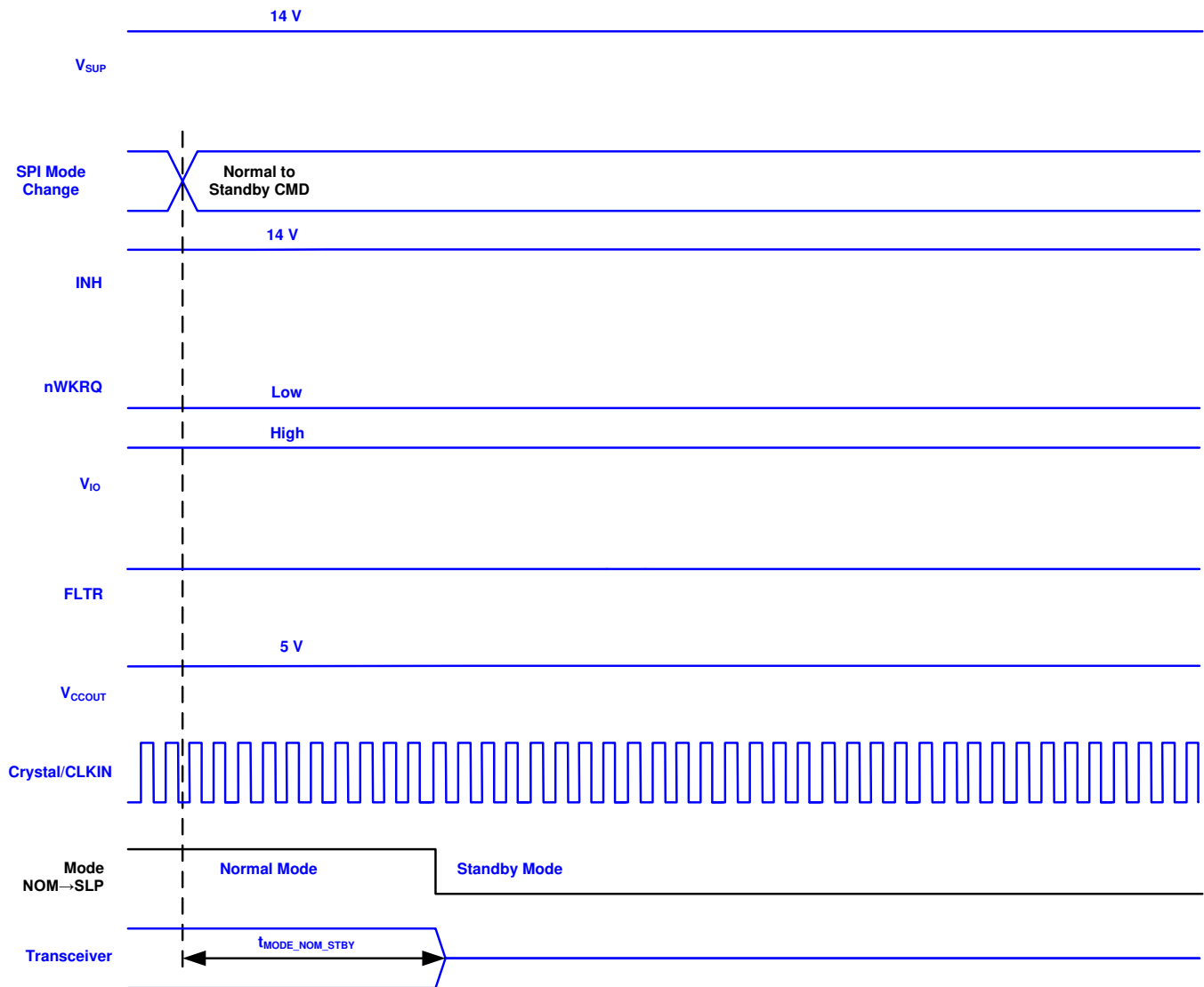
18. Normal to Standby Timing
