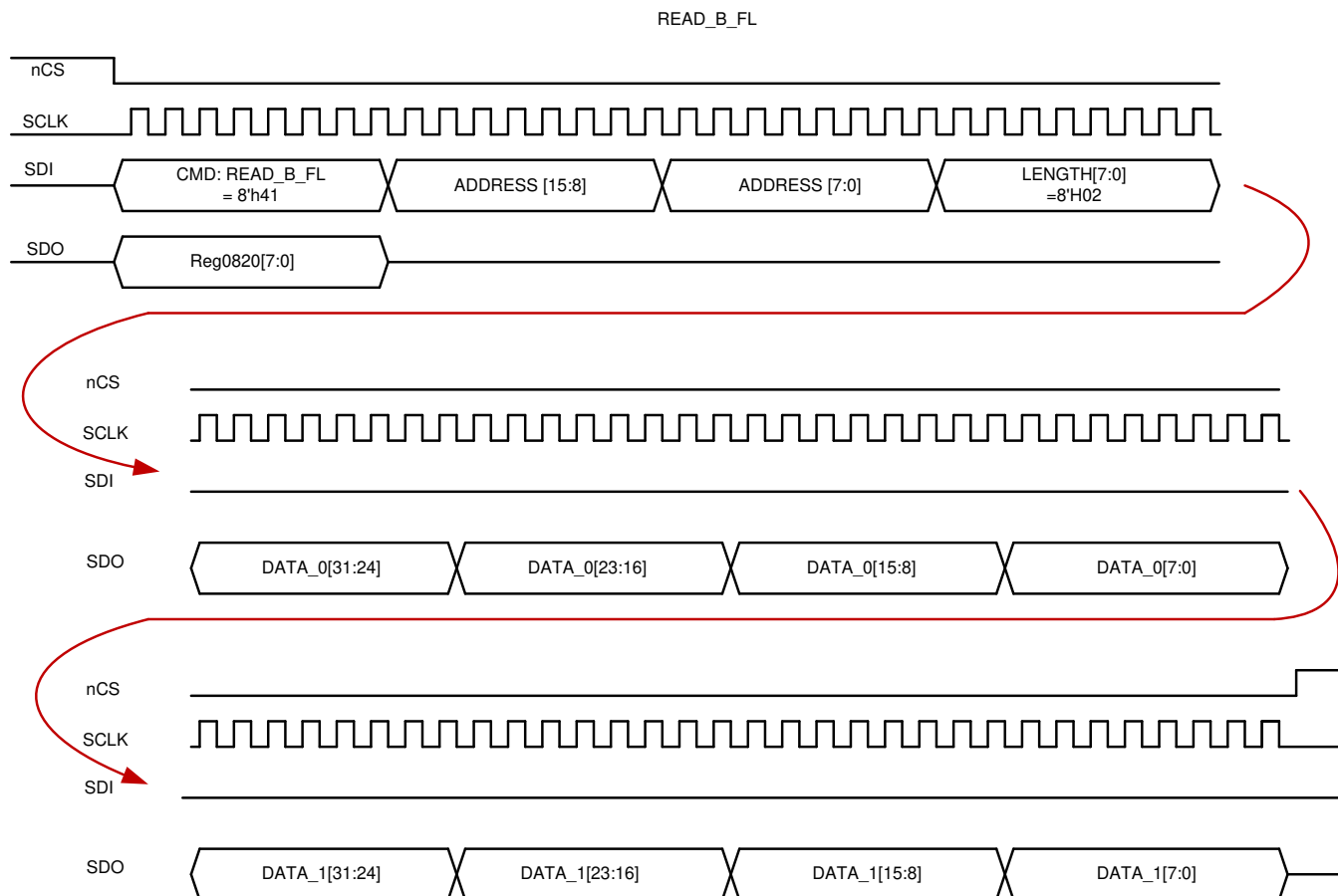
図 36. Read (Command OpCode 8h41)
