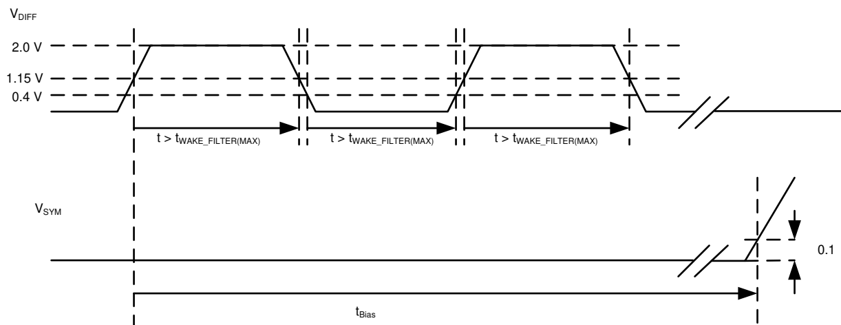
FIG 12. Test Signal Definition for Bias Reaction Time Measurement
