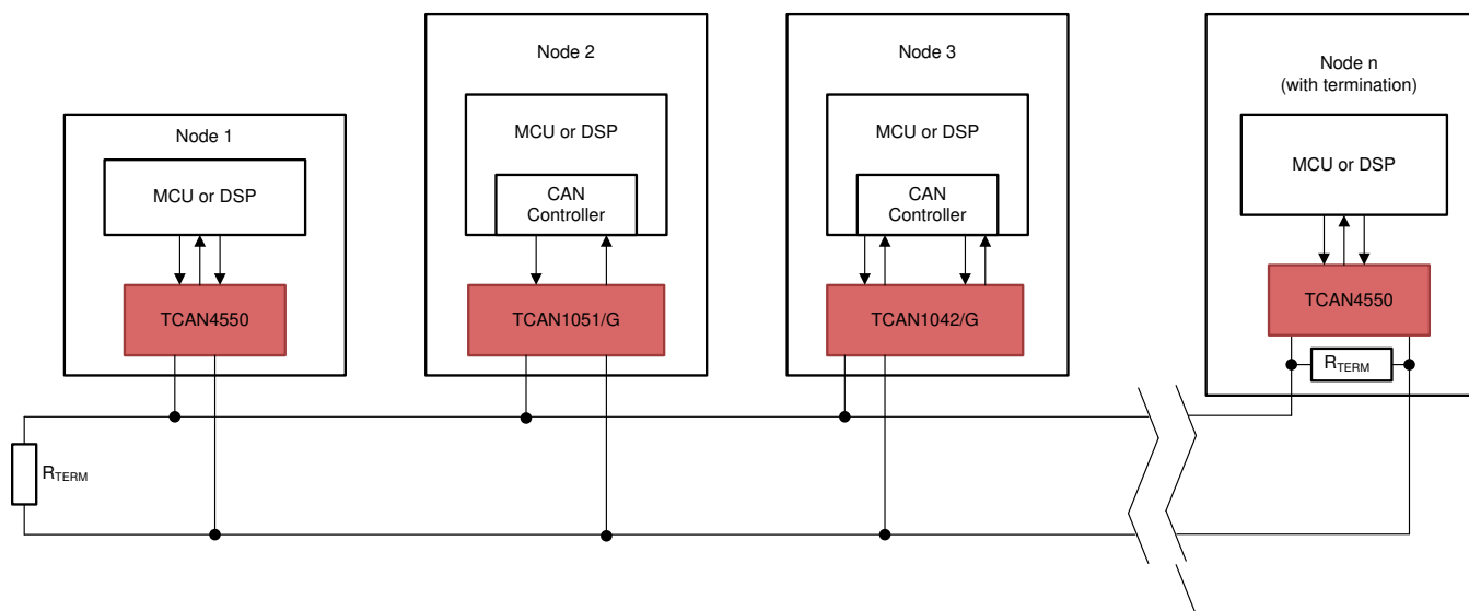
FIG 102. Typical CAN Bus
