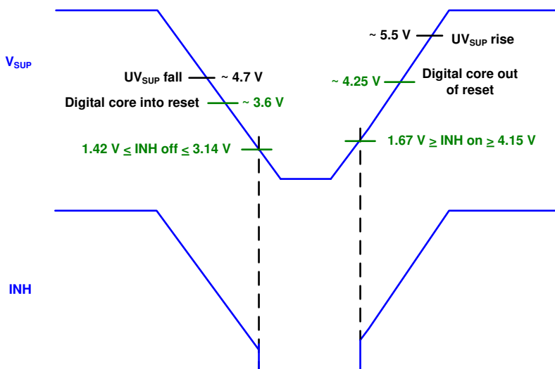
FIG 106. INH Brownout Behavior
