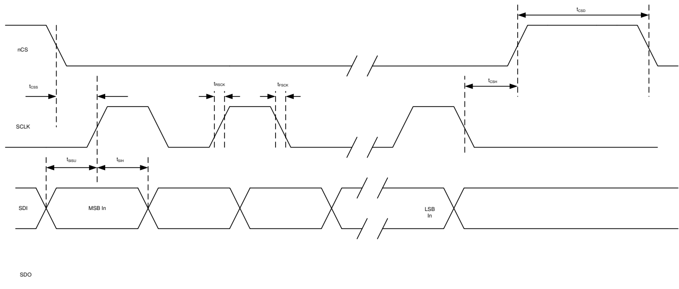
✎ 13. SPI AC Characteristic Write
