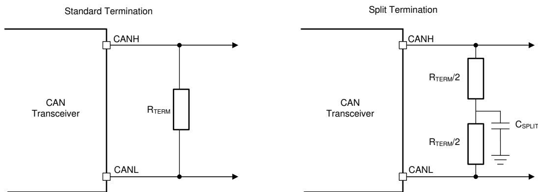
FIG 103. CAN Bus Termination Concepts
