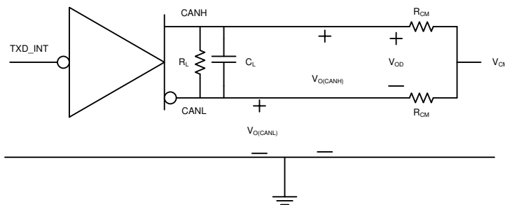
图 6. Driver Test Circuit and Measurement
