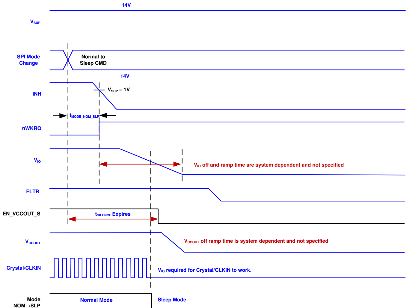
✕ 17. Normal to Sleep Timing
