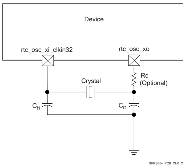
7-47. Grounding Scheme for Low-Frequency Clock
