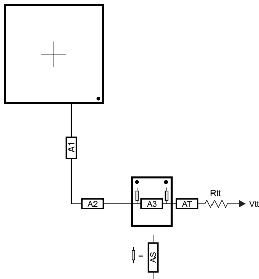
7-73. ADDR_CTRL Routing for Two Mirrored DDR3 Devices
