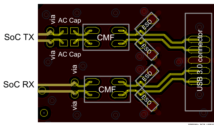
图 7-40. USB 3.0 placement diagram
