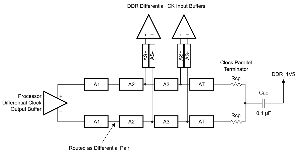
✎ 7-68. CK Topology for Two DDR3 Devices
