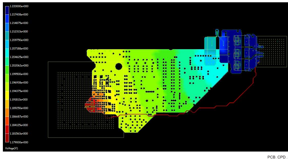
図 7-25. vdd_mpu Voltage/IR Drop [All Layers]
