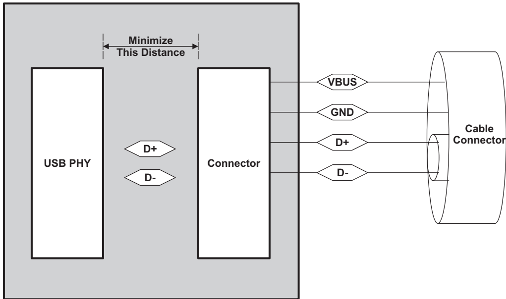
FIG 7-35. USB PHY Connector and Cable Connector
