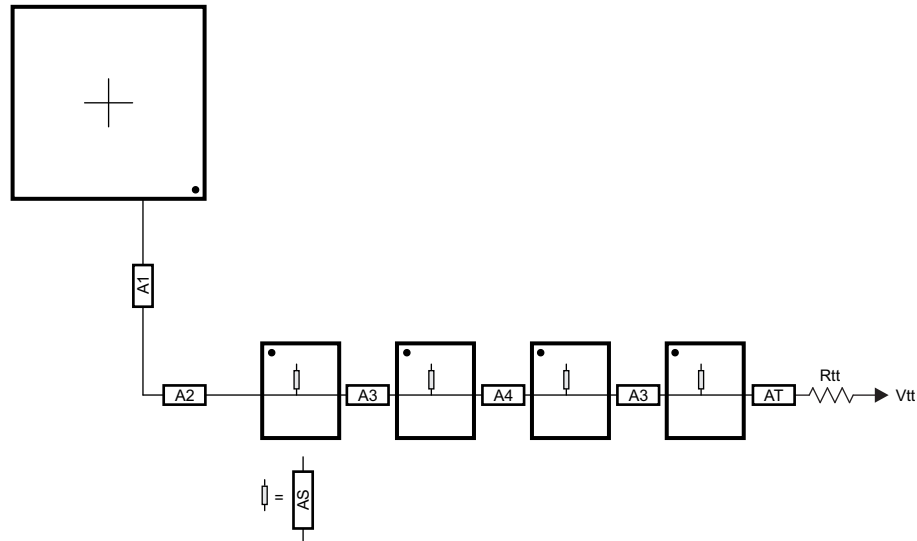
FIG 7-65. ADDR_CTRL Routing for Four Single-Side DDR3 Devices
