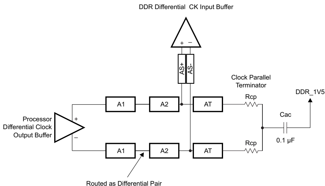
7-74. CK Topology for One DDR3 Device
