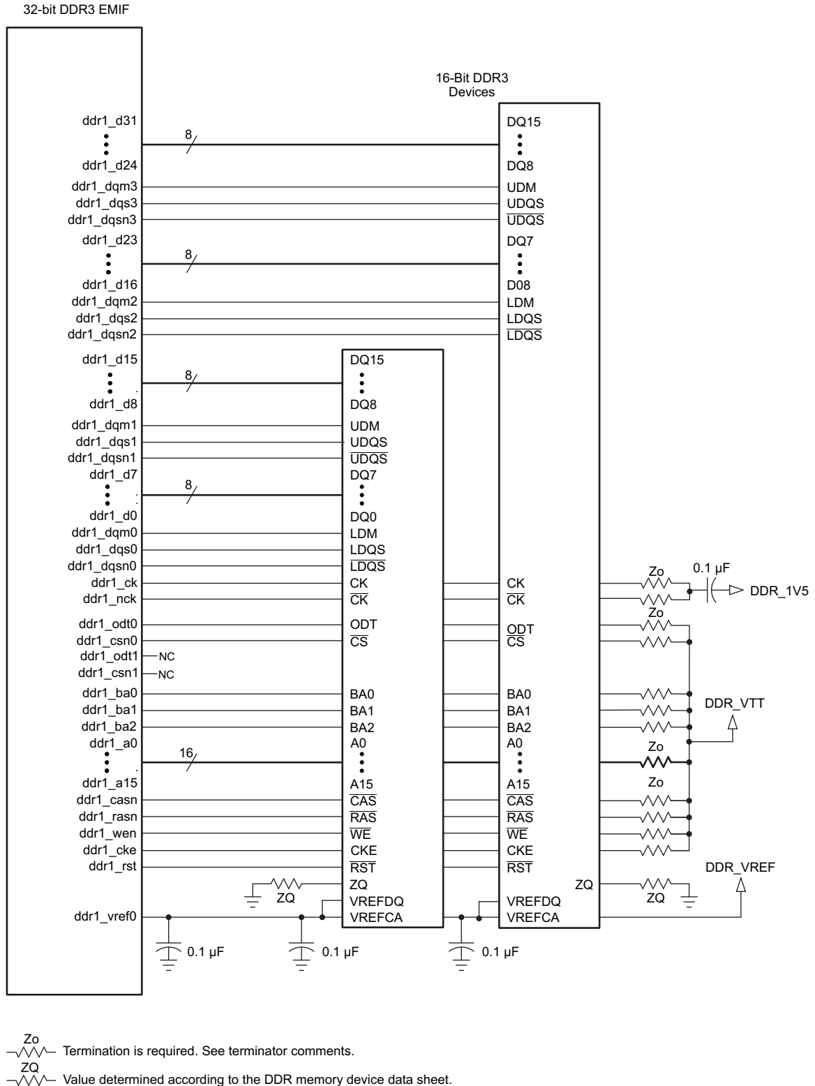
7-58. 32-Bit, One-Bank DDR3 Interface Schematic Using Two 16-Bit DDR3 Devices
