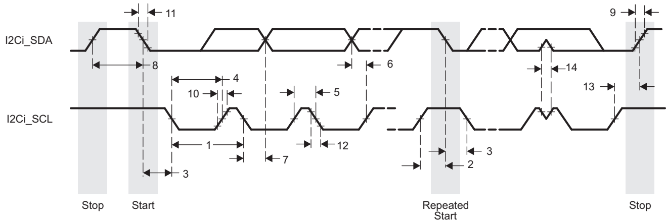
Figure 5-44. I2C Receive Timing
