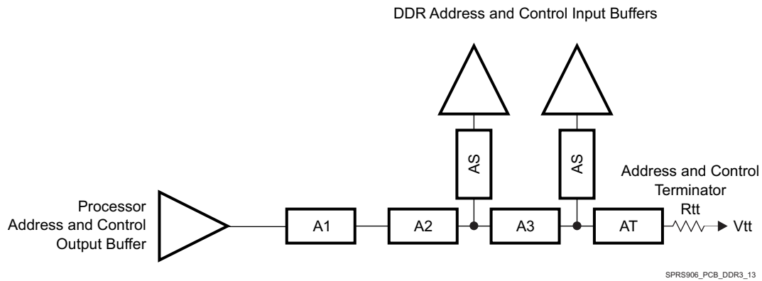
7-69. ADDR_CTRL Topology for Two DDR3 Devices
