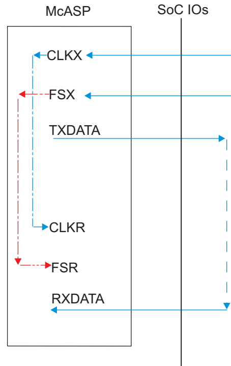
Figure 5-63. McASP1-8 CI-FI- – SYNC Mode
