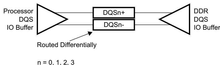
7-78. DQS Topology
