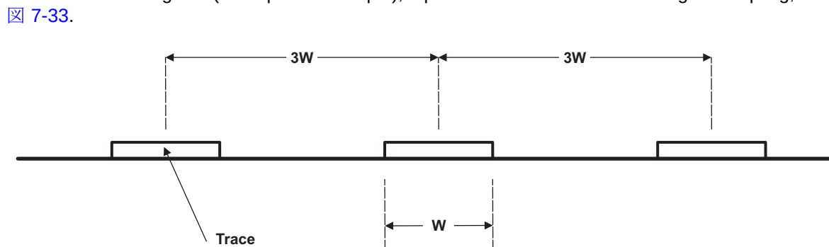
7-33. 3W Spacing Rule
