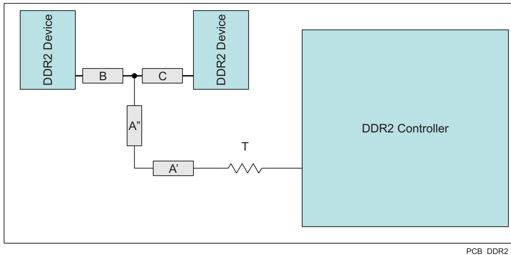
7-55. CK and ADDR_CTRL Routing and Topology
