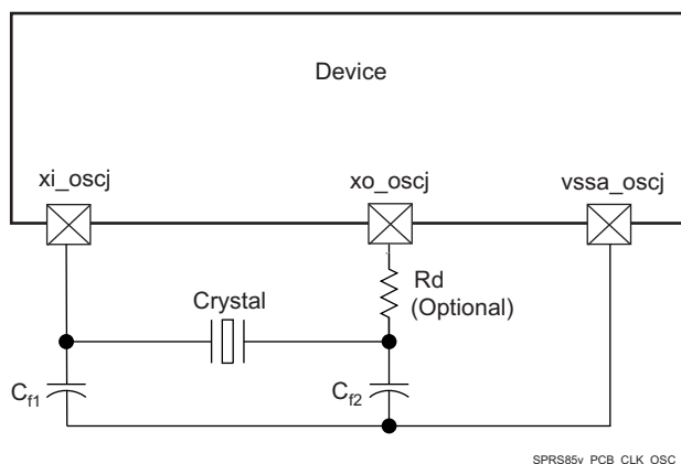
7-48. Grounding Scheme for High-Frequency Clock
