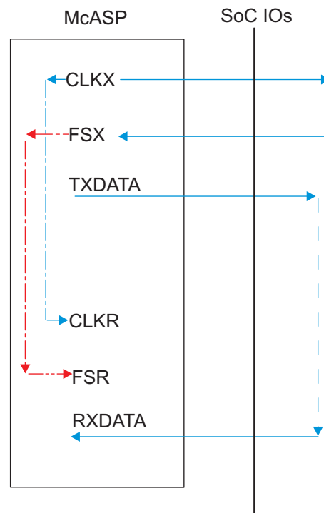
Figure 5-64. McASP1-8 CO-FI- – SYNC Mode
