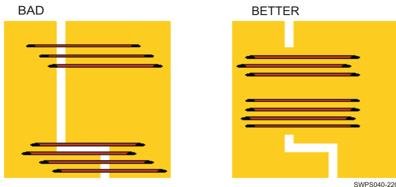
FIG 7-17. Trace Examples
