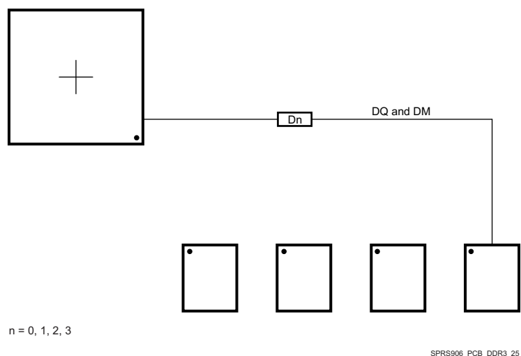
☒ 7-81. DQ/DM Routing With Any Number of Allowed DDR3 Devices
