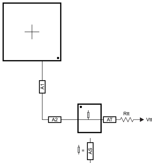
7-77. ADDR_CTRL Routing for One DDR3 Device
