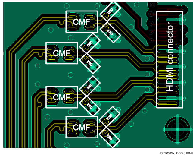
☒ 7-43. HDMI Placement Diagram
