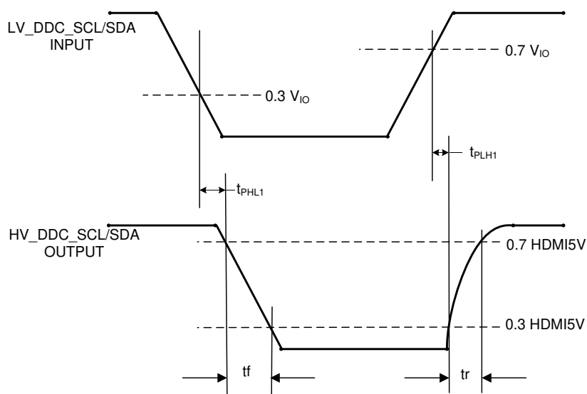
図 7-10. DDC Propagation Delay – Source to Sink
