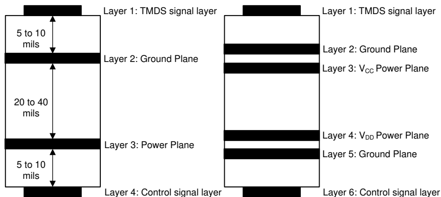
9-11. Recommended 4 or 6-Layer PCB Stack
