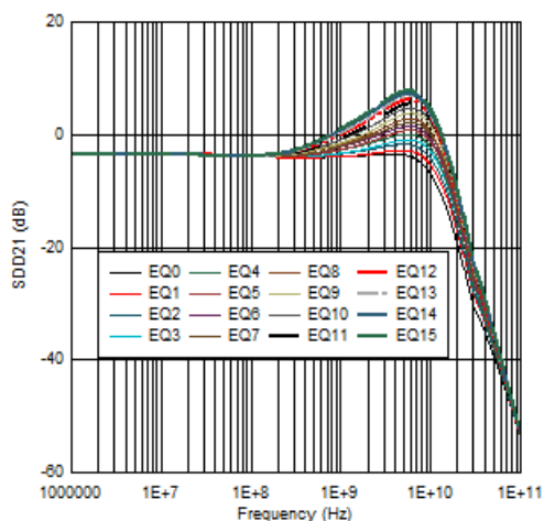
図 6-3. 12 Gbps CTLE EQ Curves with GLOBAL_DCG = 0x2 in Limited Mode
