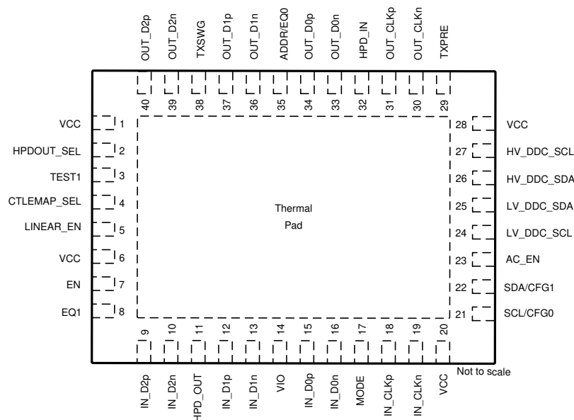
図 5-1. RNQ Package 40-Pin WQFN (Top View)
