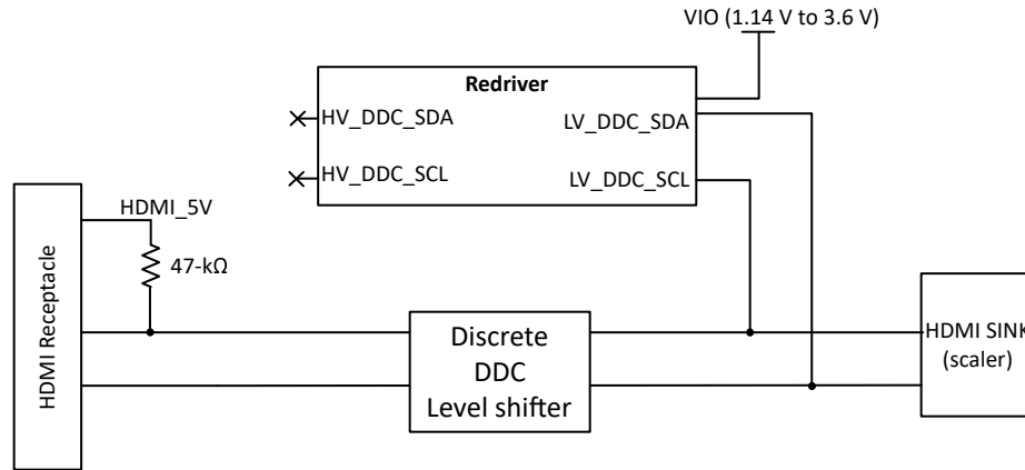
図 8-9. Sink Application: DDC Buffer Disabled and Snoop from LV DDC pins
