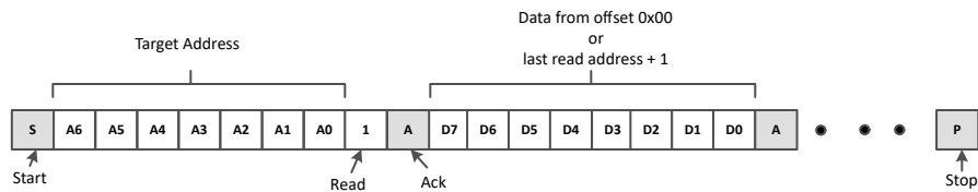
図 8-12. I 2 C Read Without Repeated Start
