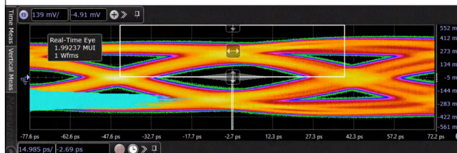
9-8. 12 Gbps Output Eye at TTP4_EQ After Pre and Post Channels
