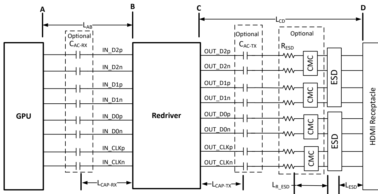
図 9-1. TDP1204 in Source Side Application
