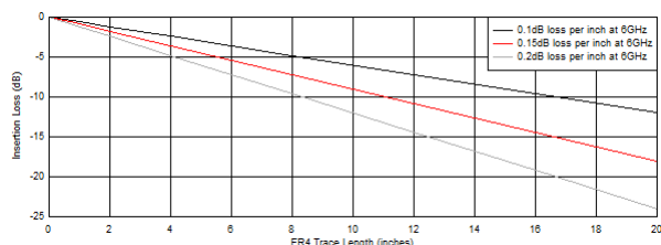
9-3. FR4 Trace Insertion Loss at 6 GHz
