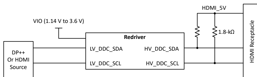
図 8-5. Source Application: DDC Buffer Enabled
