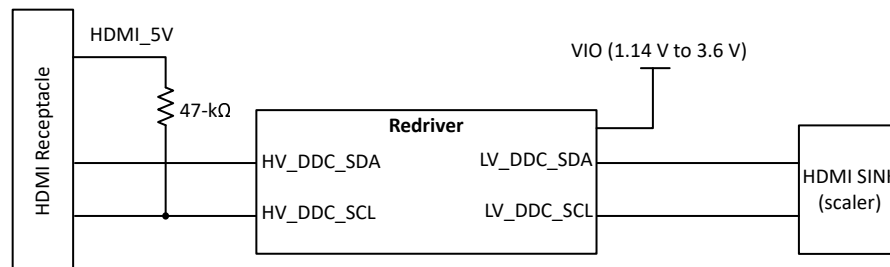
図 8-8. Sink Application: DDC Buffer Enabled
