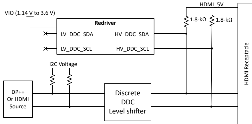
図 8-6. Source Application: DDC Buffer Enabled and Snoop from HV DDC pins
