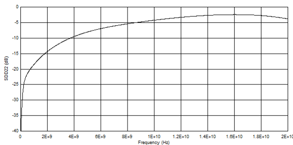
図 6-5. Output Differential Return Loss (SDD22)
