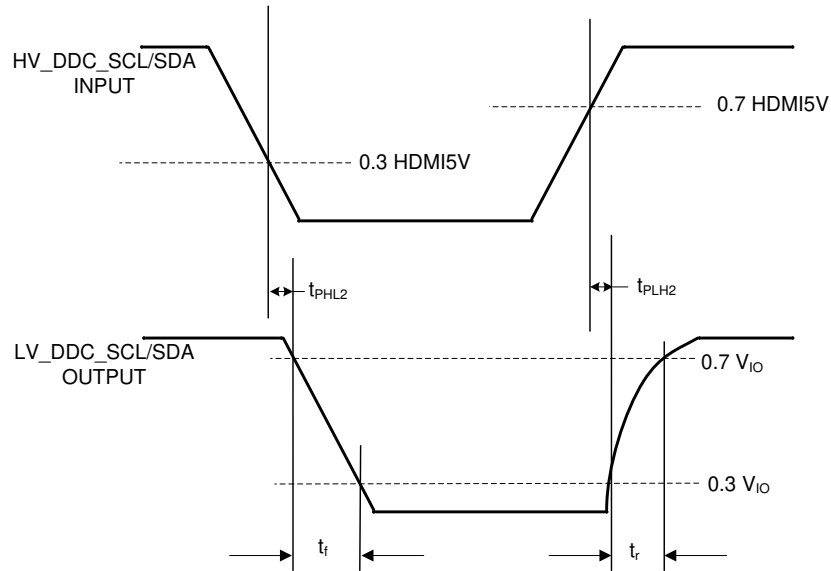
図 7-11. DDC Propagation Delay – Sink to Source
