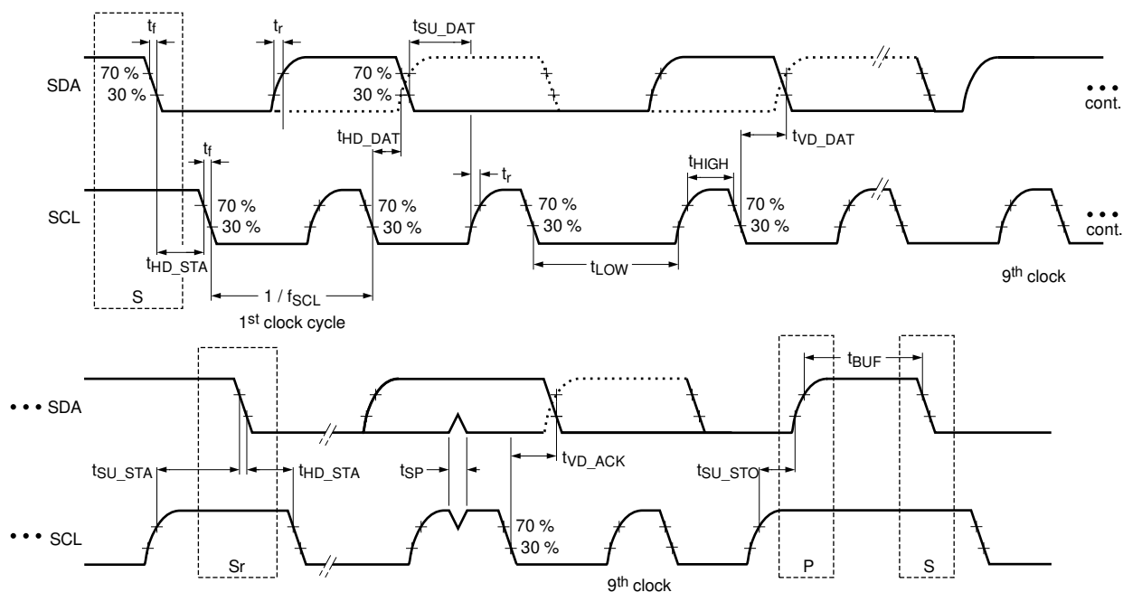
図 7-9. I 2 C SCL and SDA Timing
