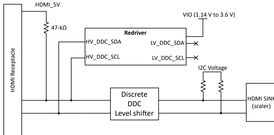
図 8-10. Sink Application: DDC Buffer Enable and Snoop from HV DDC pins
