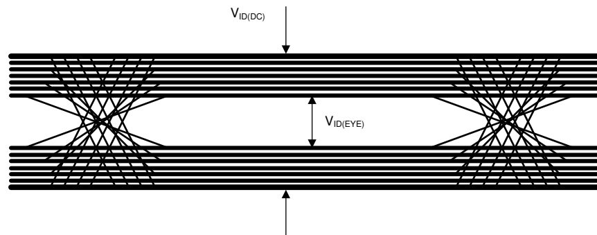
図 7-12. V_{ID(DC)} and V_{ID(EYE)}
