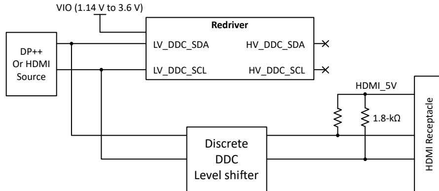
図 8-7. Source Application: DDC Buffer Disabled and Snoop from LV DDC pins
