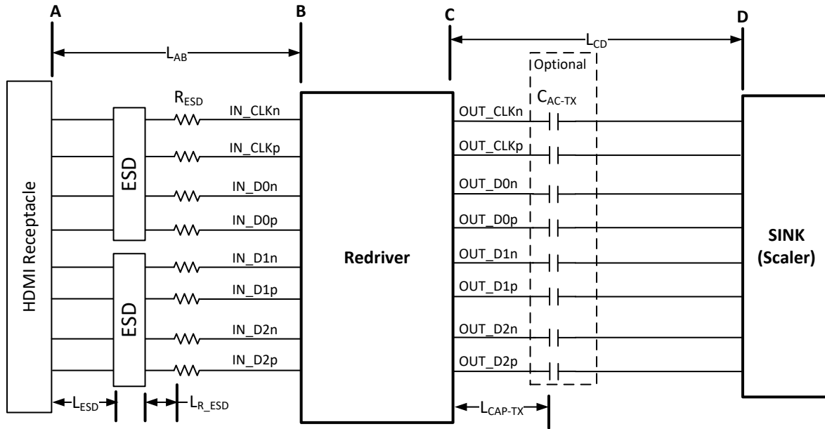
図 9-9. TDP1204 in Sink Side Application
