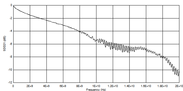
9-5. Post-Channel Insertion Loss at TTP4
