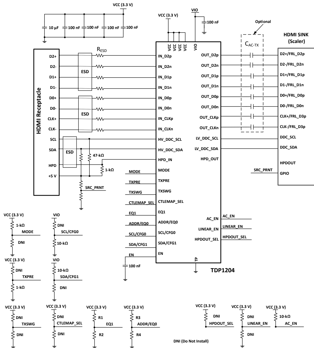
9-10. TDP1204 in Sink Application Schematics
