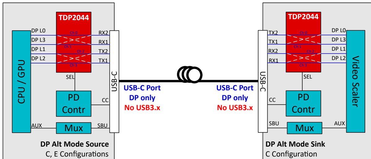
図 7-1. Typical Application
