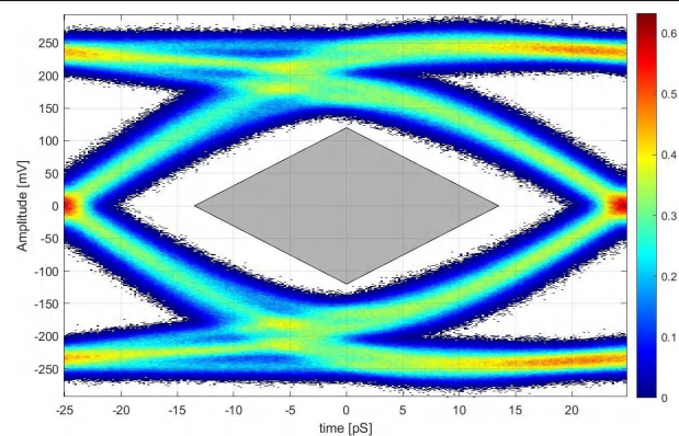
Figure 7-6. DP 2.1 Tx Compliance Eye Diagram at TP3_EQ with TDP2044 for Signal Conditioning
