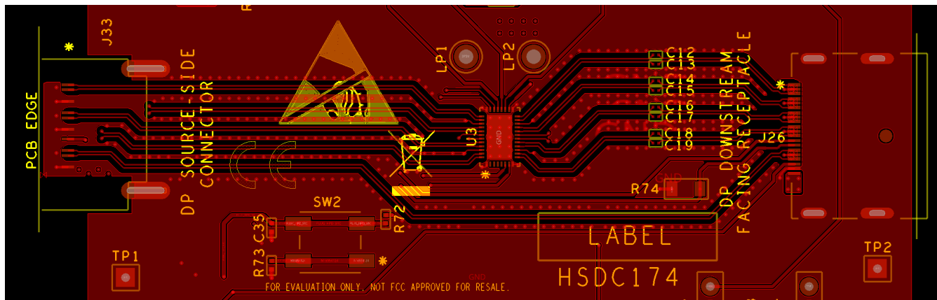
図 7-7. TDP2044 Layout Example – Sub-Section of TI Evaluation Board with DP Connectors
