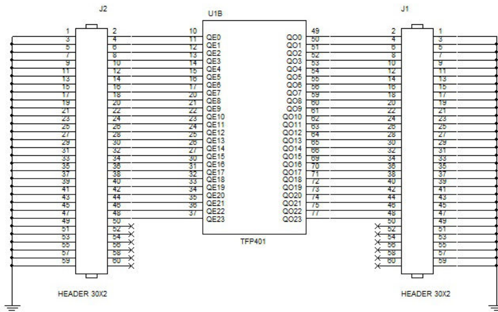
FIG 10-2. Data and Control Signals Design
