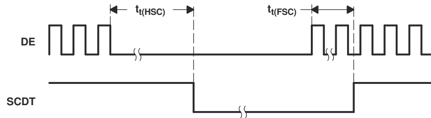
FIG 8-12. Time Between DE Transitions to SCDT Low and SCDT High
