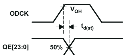
8-5. ODCK High to QE[23:0] Staggered Data Output
