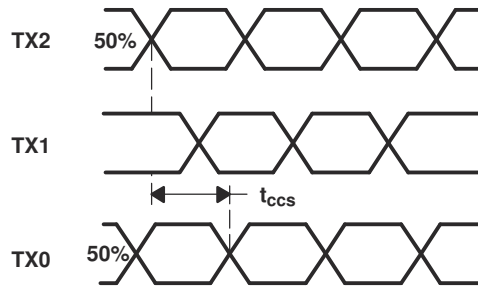
FIG 8-11. Analog Input Channel-to-Channel Skew
