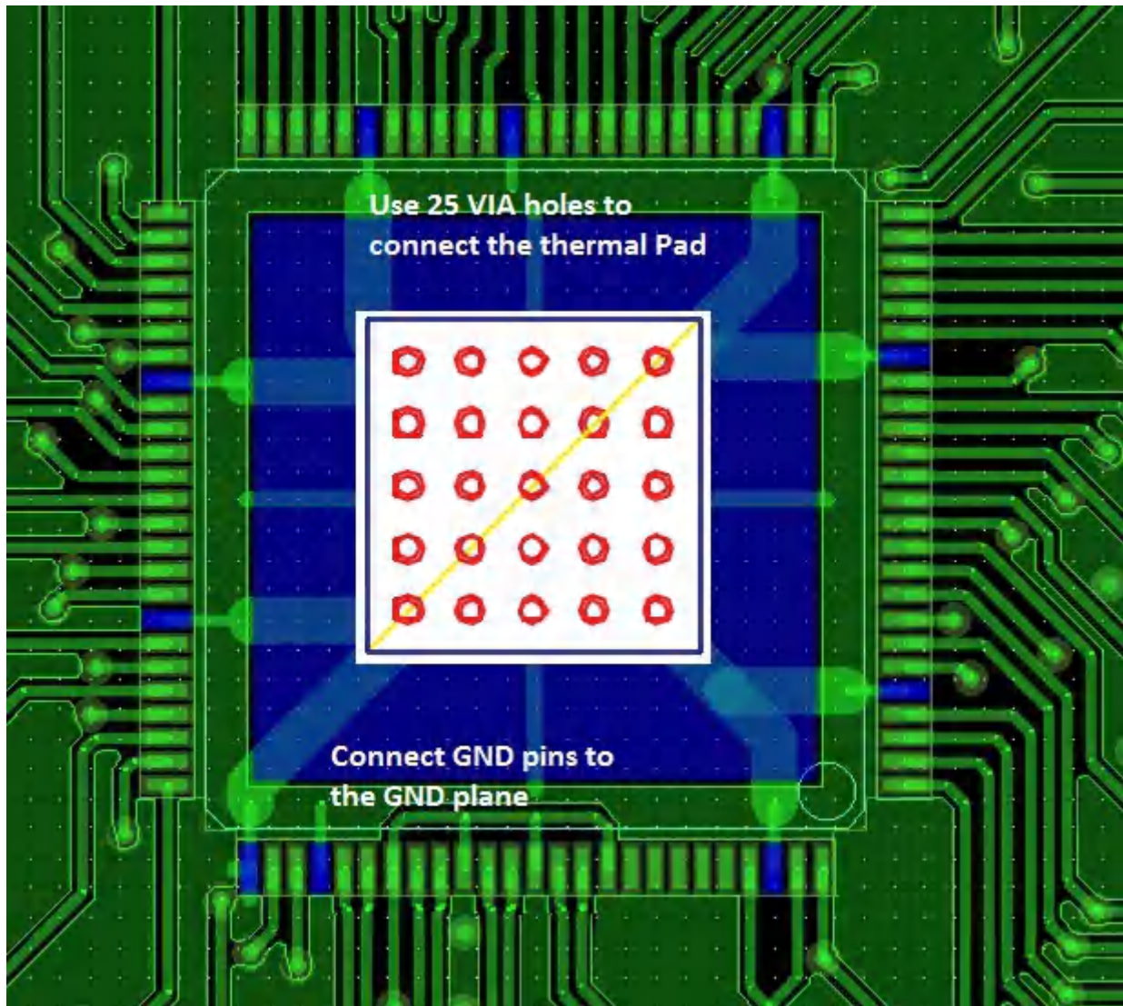
✎ 12-4. Ground Routing
