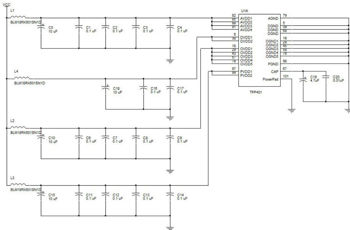
10-4. Power Supplies Decoupling Design
