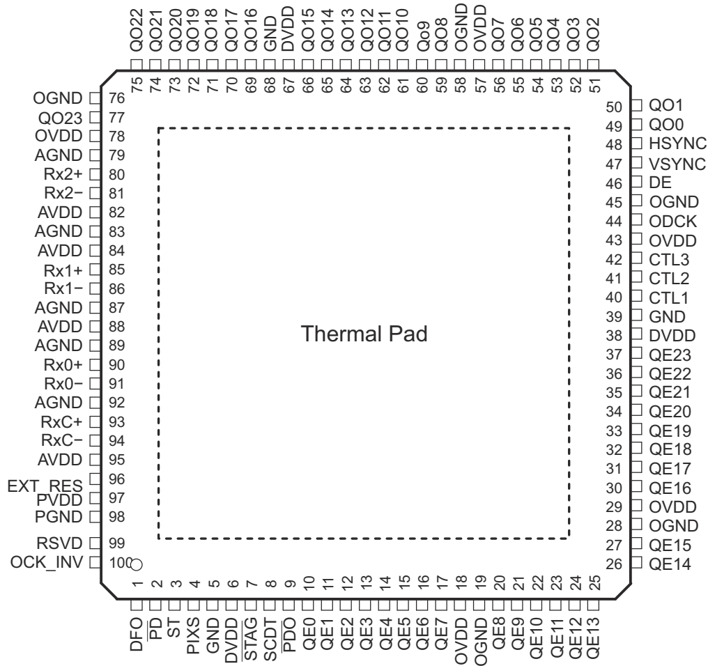
図 6-1. PZP Package, 100-Pin HTQFP (Top View)
