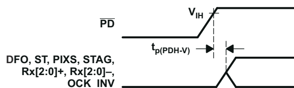
8-9. Delay From \overline{\text{PD}} Low to High Before Inputs Are Active
