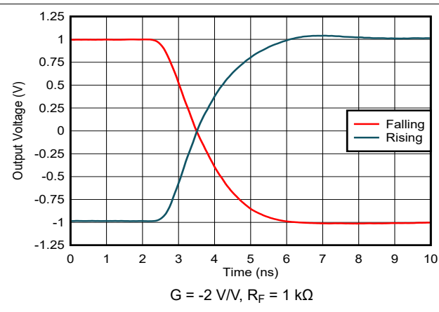
7-35. Settling Time
