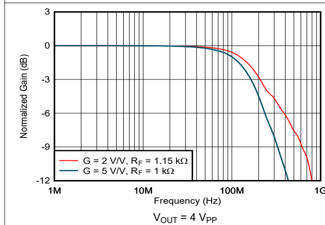
7-34. Noninverting Large-Signal Frequency Response
