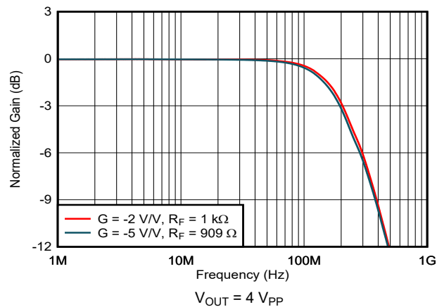
7-6. Inverting Large-Signal Frequency Response
