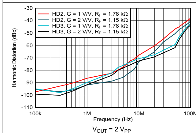
7-36. Harmonic Distortion vs Frequency
