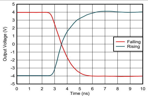
7-18. Settling Time
