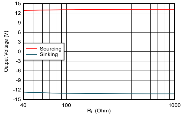
7-20. Output Voltage vs Load Resistance
