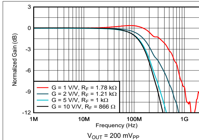
7-32. Noninverting Small-Signal Frequency Response
