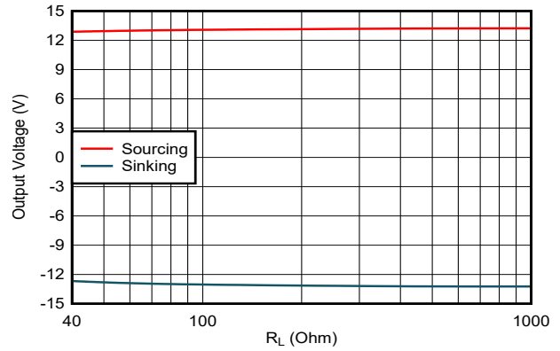
FIG 7-20. Output Voltage vs Load Resistance
