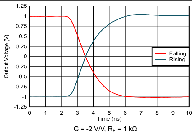
7-35. Settling Time
