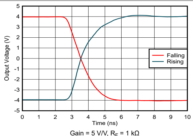
Figure 7-18. Settling Time
