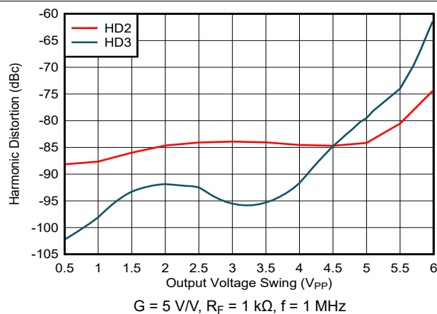
7-37. Harmonic Distortion vs Output Voltage Swing
