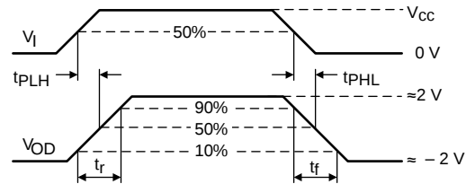
FIG 13. Measurement of Driver Differential Output Rise and Fall Times and Propagation Delays
