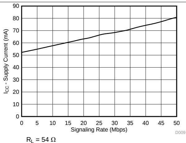
Figure 9. THVD1550 Supply Current vs Signal Rate
