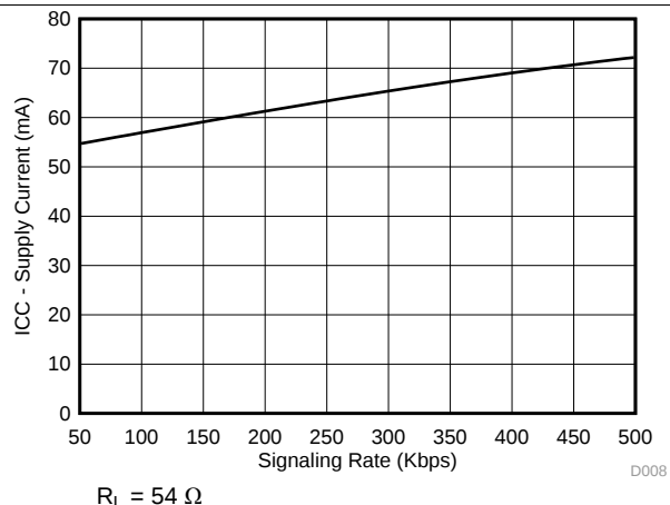
Figure 8. THVD1510 Supply Current vs Signal Rate
