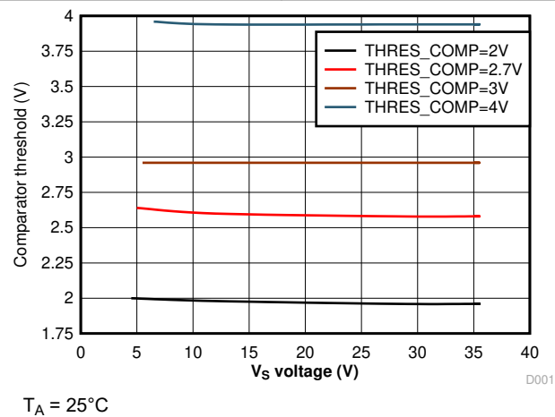
FIG 6-3. Comparator Threshold vs. V_S Voltage
