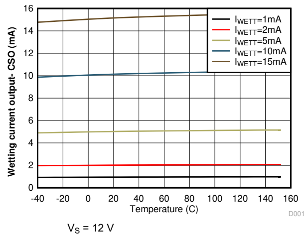
FIG 6-2. Wetting current output - CSO vs. Temperature
