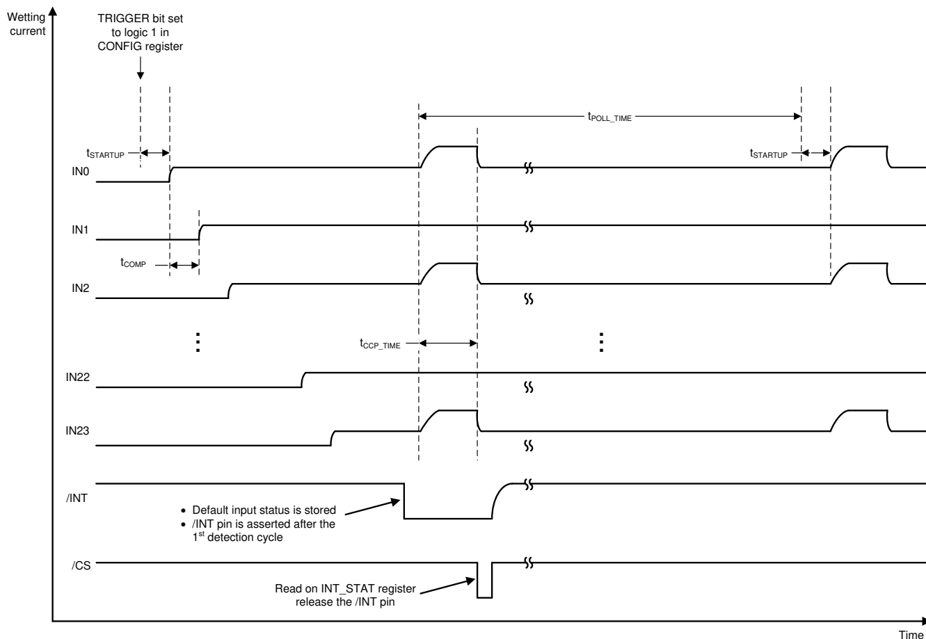
8-15. Continue Mode With CCP Enabled
