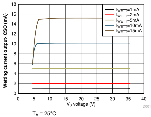
FIG 6-1. Wetting current output - CSO vs. V_S Voltage
