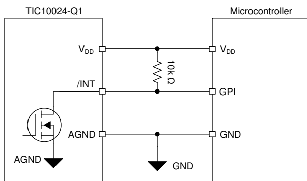
FIG 8-4. \overline{\text{INT}} Connection Example #1
