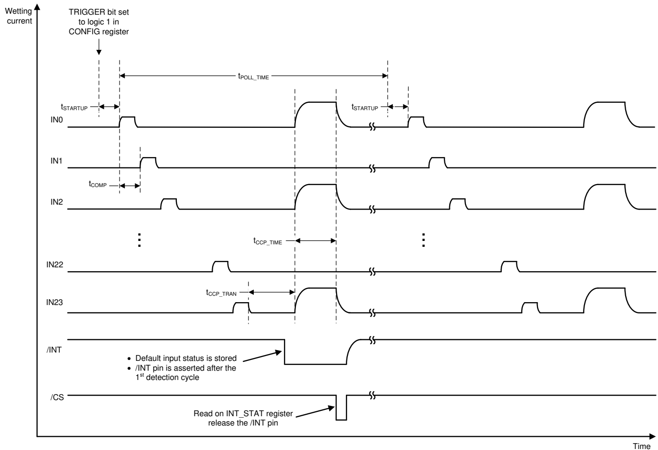
8-14. Polling With CCP Enabled
