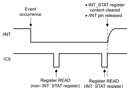
FIG 8-5. Static \overline{\text{INT}} Assertion Scheme
