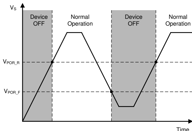
FIG 8-1. V_S is Lowered Below The POR threshold, Then Ramped Back Up To Complete A POR Cycle
