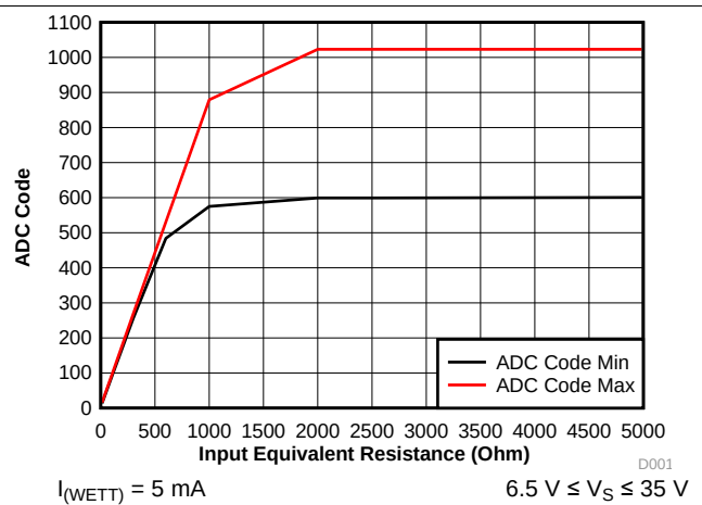
FIG 6. ADC Code vs. Equivalent Resistance at INx
