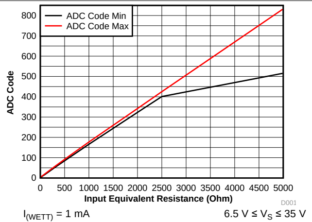
FIG 4. ADC Code vs. Equivalent Resistance at INx
