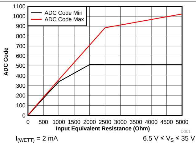
FIG 5. ADC Code vs. Equivalent Resistance at INx
