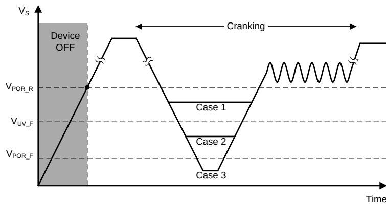
FIG 13. TIC12400 Operation At Various V_S Voltage Levels
