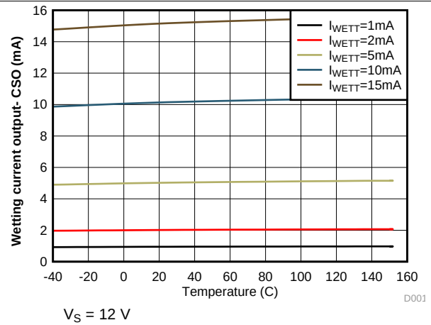
FIG 2. Wetting Current Output - CSO vs. Temperature
