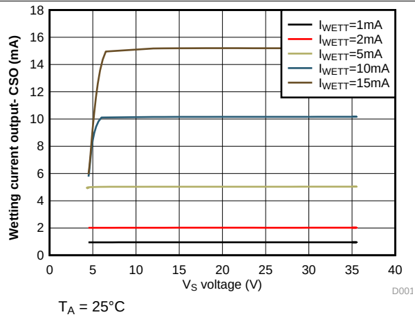
FIG 1. Wetting Current Output - CSO vs. V_S Voltage
