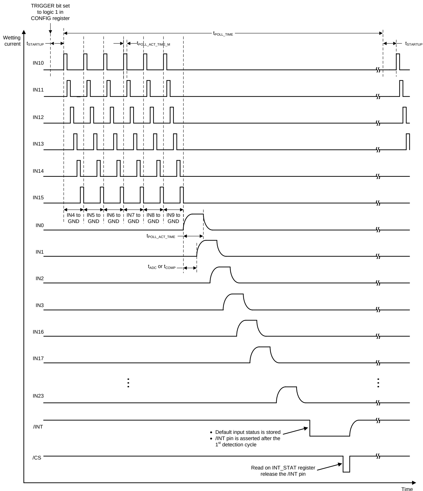
26. Polling Scheme for 6x6 Matrix Inputs
