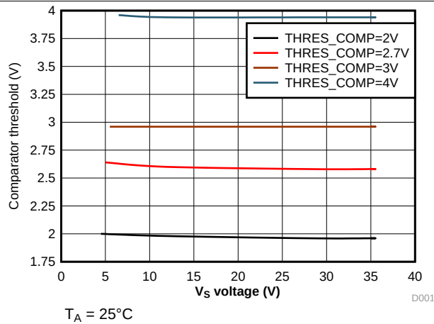
FIG 3. Comparator Threshold vs. V_S Voltage
