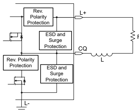
Figure 9-3. N-Switch Mode
