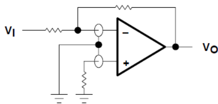
(b) INVERTING AMPLIFIER
