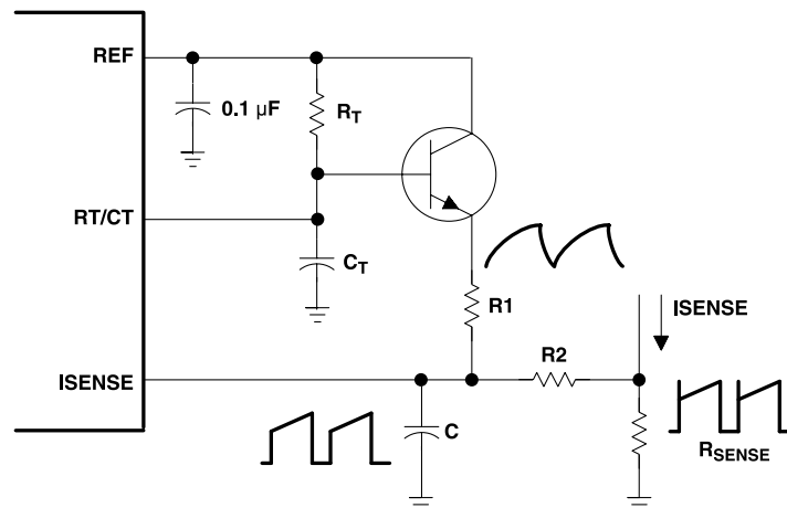
Figure 6-2. Slope Compensation
