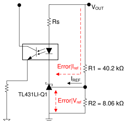
26. Feedback Quiescent Current
