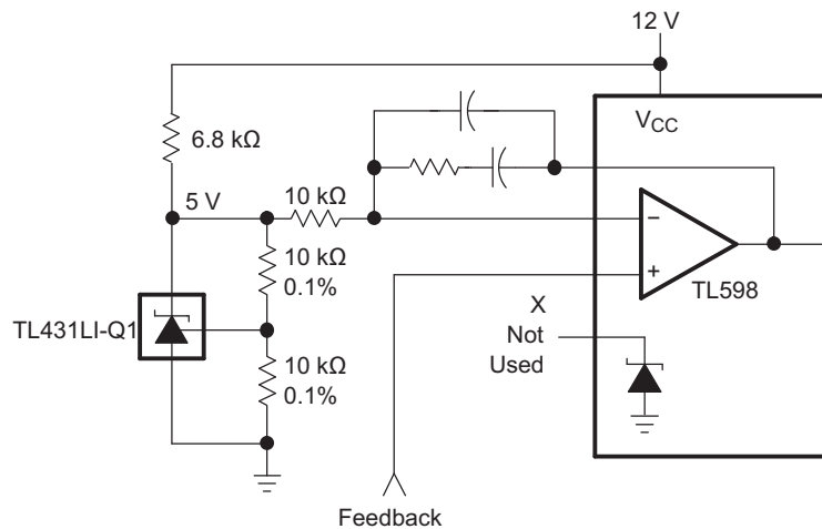
FIG 33. PWM Converter With Reference
