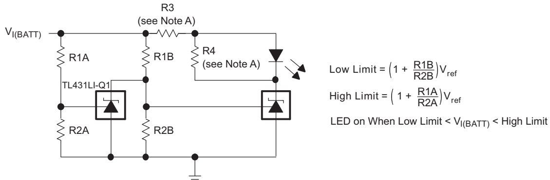
FIG 34. Voltage Monitor
