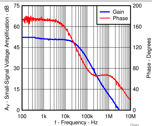
FIG 6. Small-Signal Voltage Amplification versus Frequency
