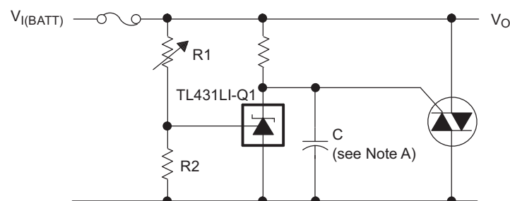
FIG 30. Crowbar Circuit
