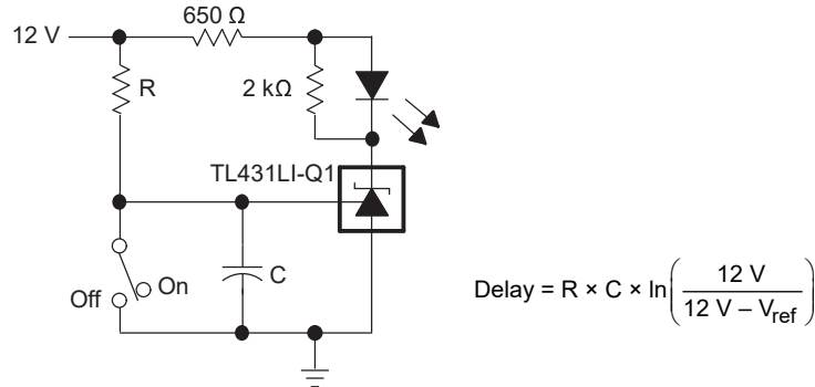
FIG 35. Delay Timer
