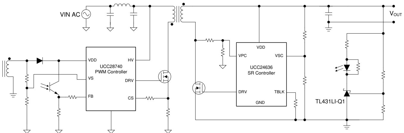
☒ 25. Isolated Flyback with Optocoupler
