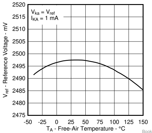
FIG 1. Reference Voltage versus Free-Air Temperature
