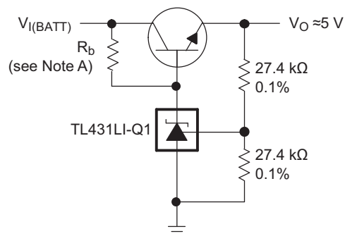
FIG 32. Efficient 5-V Low-Dropout (LDO) Regulator Configuration
