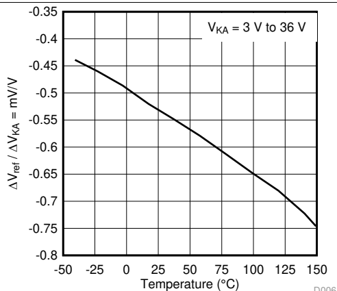
FIG 5. Ratio of Delta Reference Voltage to Delta Cathode Voltage versus Free-Air Temperature
