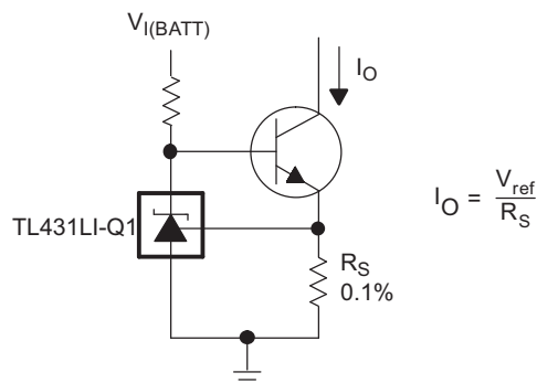
FIG 37. Precision Constant-Current Sink
