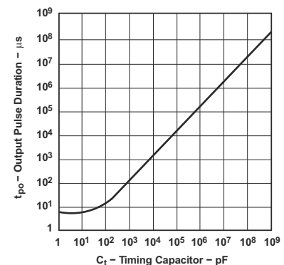
Figure 6-6. Output Pulse Duration vs Timing Capacitor
