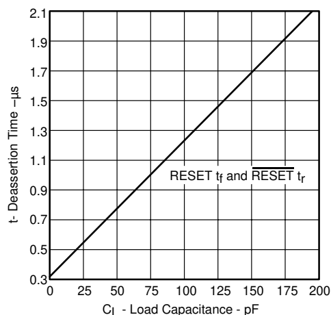
6-6. Deassertion Time vs Load Capacitance
