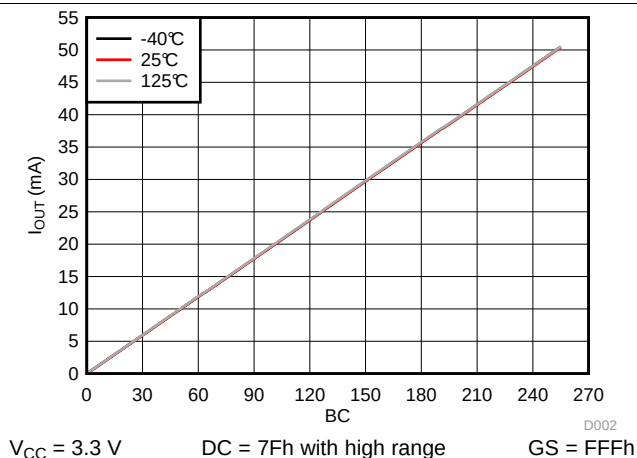
FIG 20. I_{OUT} vs Brightness Control at Different Ambient Temperatures
