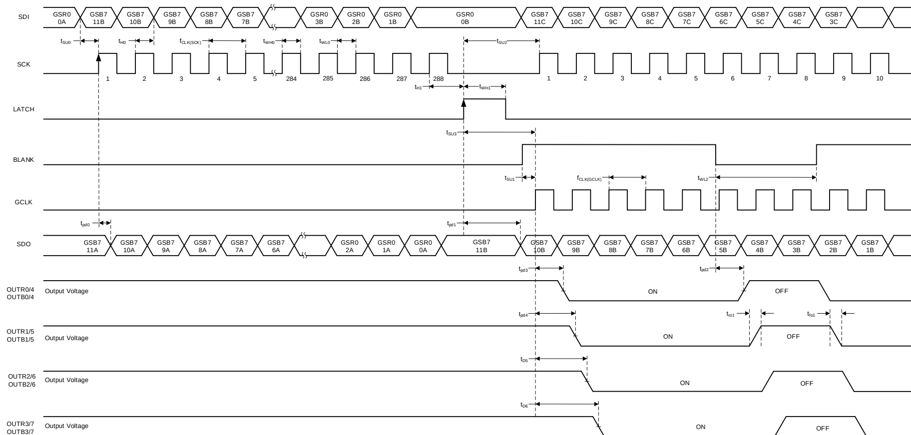
1. Grayscale Data (GS) Write
