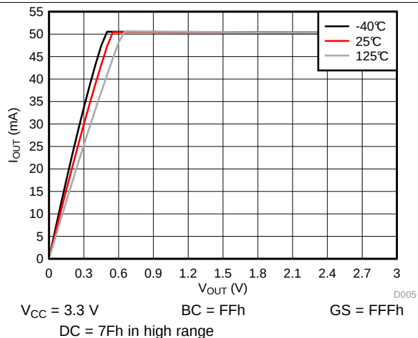
FIG 16. I_{OUT} vs V_{OUT}
