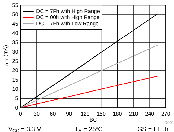
FIG 19. I_{OUT} vs Brightness Control in Different DC Ranges
