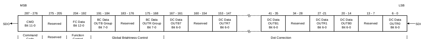
Figure 26. FC-BC-DC Register
