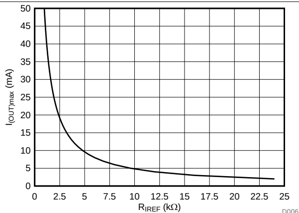
FIG 15. I_{OUTmax} vs R_{REF}
