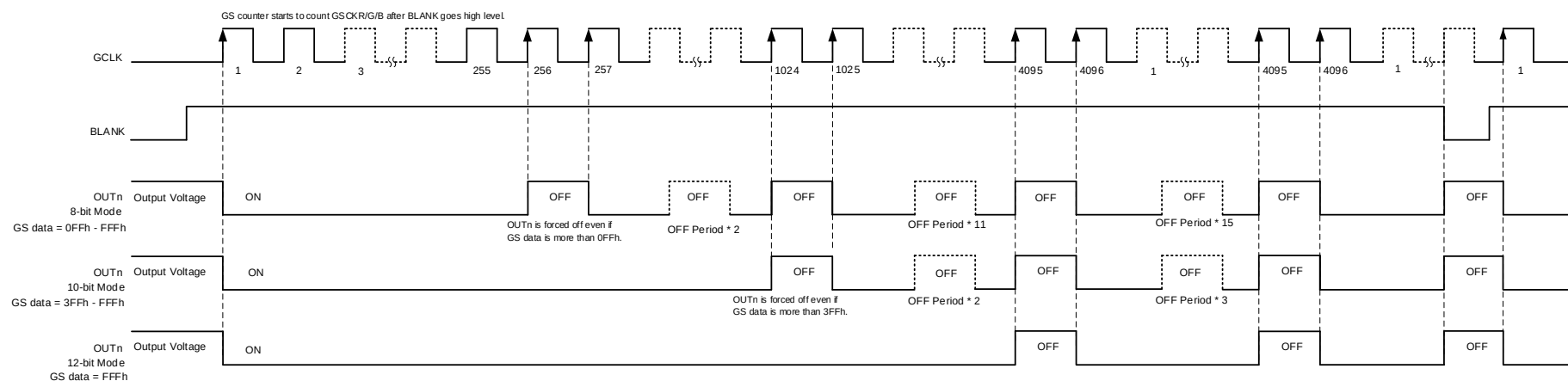
图 13. 8-, 10-, 12-Bit Mode PWM Counter With Auto-Repeat Mode
