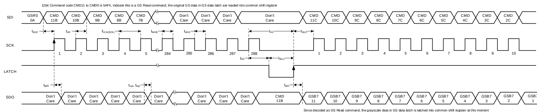
3. Grayscale (GS) Data Read
