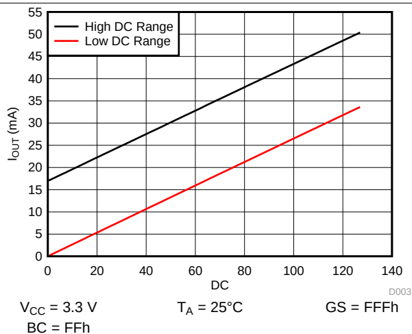
FIG 17. I_{OUT} vs Dot Correction in Different DC Ranges
