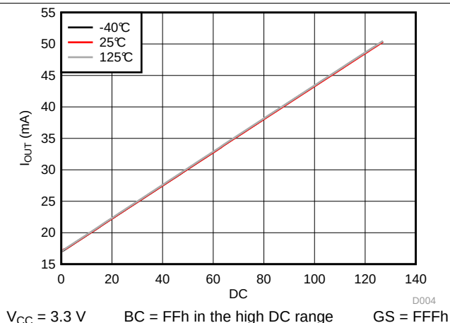
FIG 18. I_{OUT} vs Dot Correction at Different Ambient Temperatures
