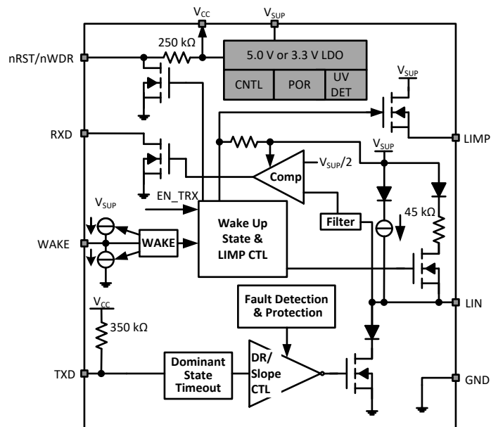
FIG 9-1. Transceiver plus VREG Functional Block Diagram
