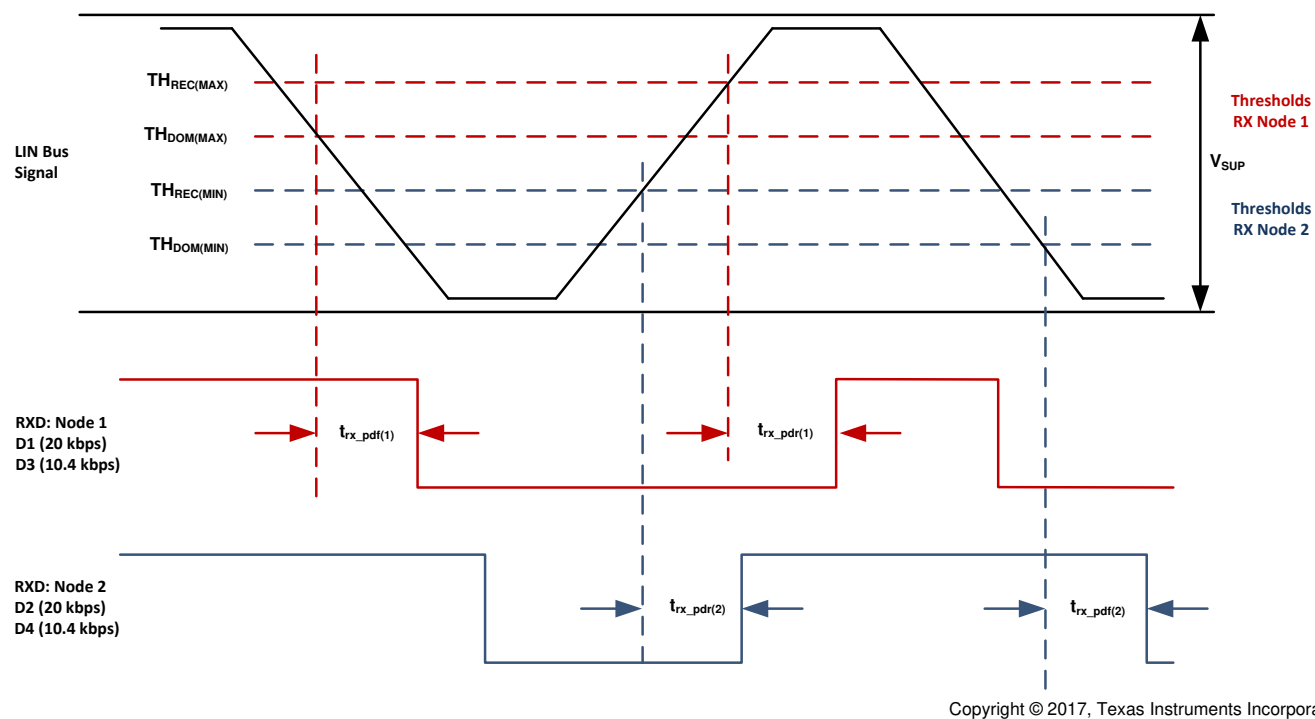
8-14. Propagation Delay
