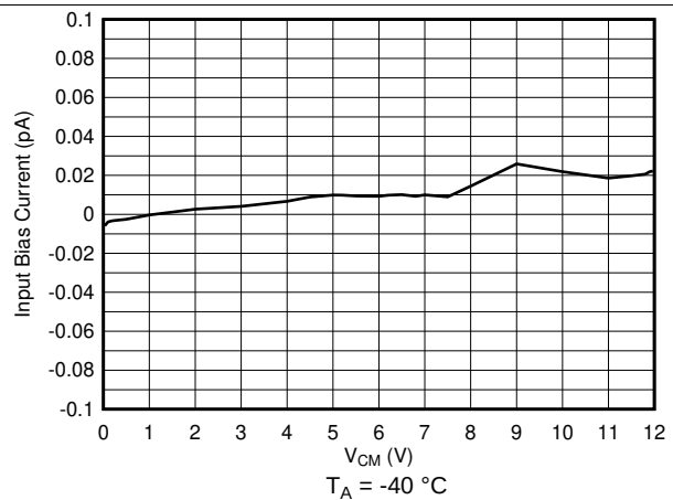
FIG 12. Input Bias Current vs. Common Mode, -40°C
