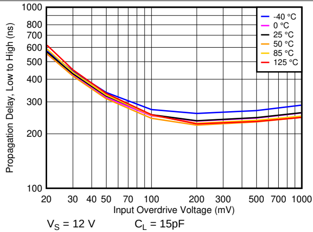
FIG 39. T_{PLH} Response Time vs. Overdrive at 12V
