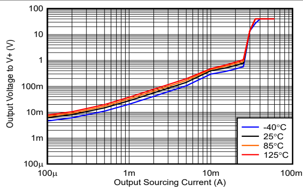
5-11. Output Voltage vs. Sourcing Current, 40V, Push-Pull only
