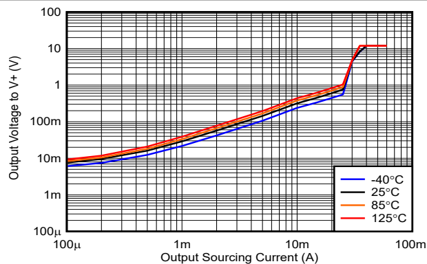
5-9. Output Voltage vs. Sourcing Current, 12V, Push-Pull only
