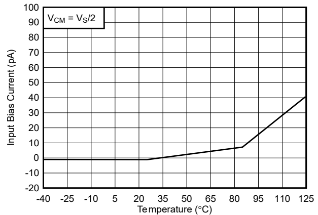
図 5-6. Bias Current vs. Temperature, 40V
