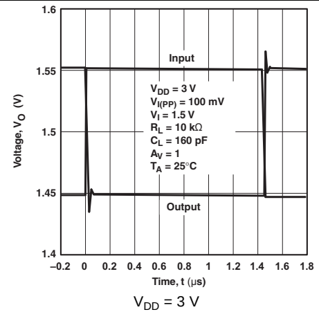
Figure 46. Inverting Small Signal
