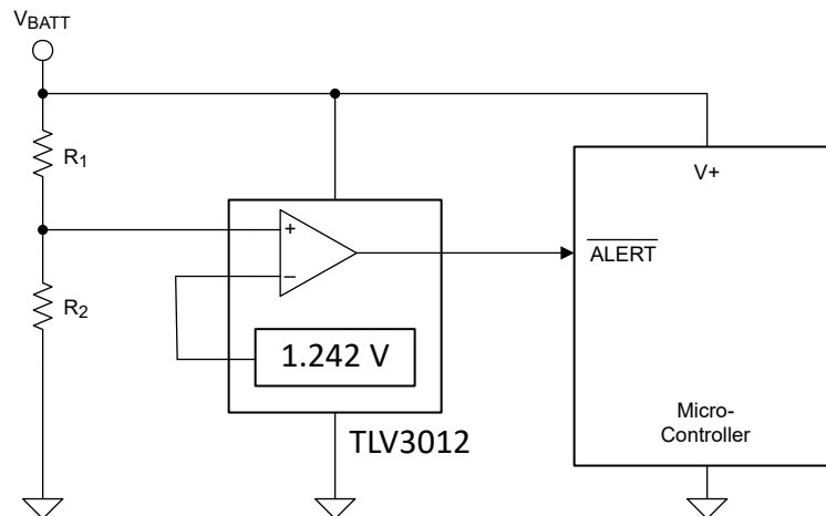
10-3. Under-Voltage Detection
