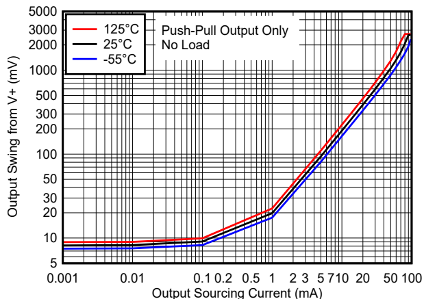
図 6-4. Output Swing vs. Output Sourcing Current - 3.3V
