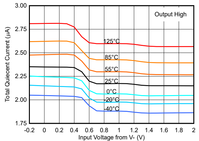
図 6-10. Supply Current vs. Common Mode - 1.8V
