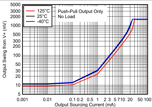
図 6-2. Output Swing vs. Output Sourcing Current - 1.8V
