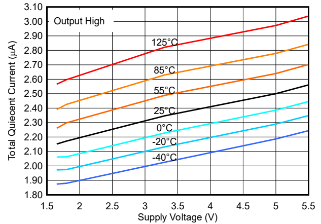
図 6-8. Supply Current vs. Supply Voltage
