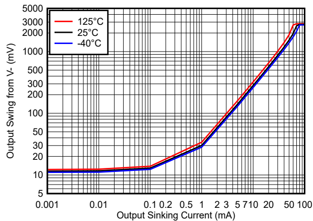
図 6-3. Output Swing vs. Output Sinking Current - 3.3V
