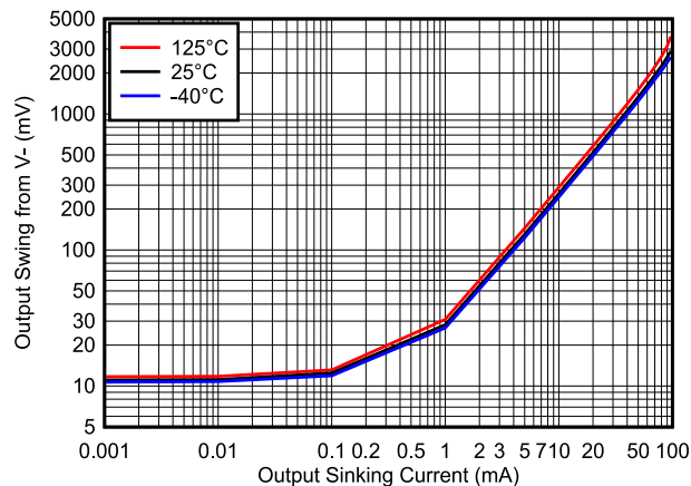
図 6-5. Output Swing vs. Output Sinking Current - 5V
