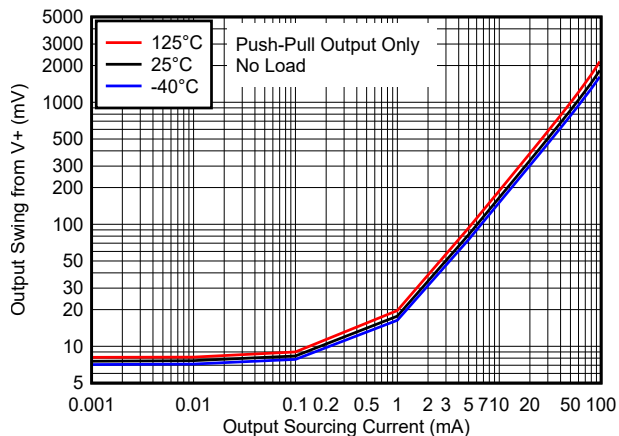
図 6-6. Output Swing vs. Output Sourcing Current - 5V
