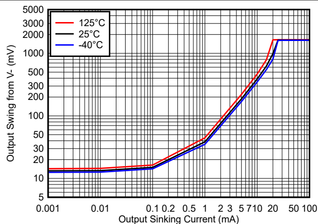
図 6-1. Output Swing vs. Output Sinking Current - 1.8V
