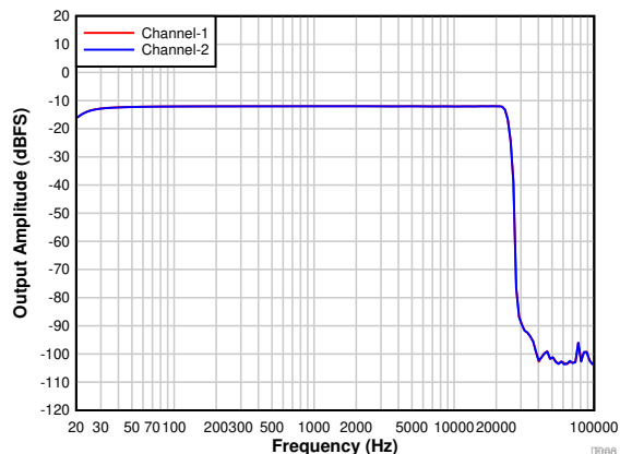
Figure 7-11. Frequency Response With a -12-dBr Input
