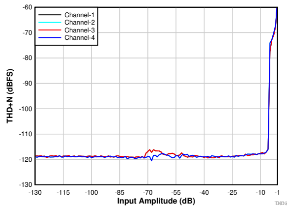
Figure 7-16. PDM Input THD+N vs Input Amplitude
