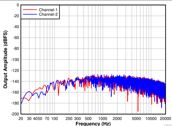
Figure 7-13. FFT With Idle Input
