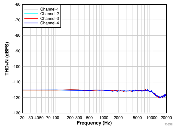
Figure 7-17. PDM Input THD+N vs Input Frequency With a -20-dBr Input
