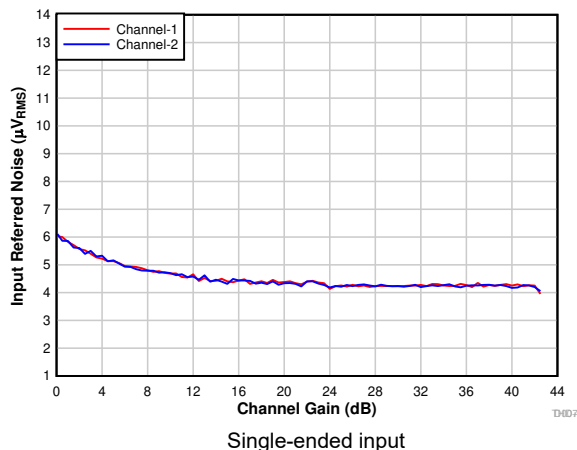
Figure 7-10. Input-Referred Noise vs Channel Gain
