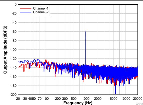
图 9-2. FFT With a -60-dBr Input
