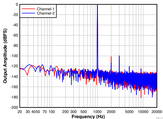
Figure 7-15. FFT With a -1-dBr Input
