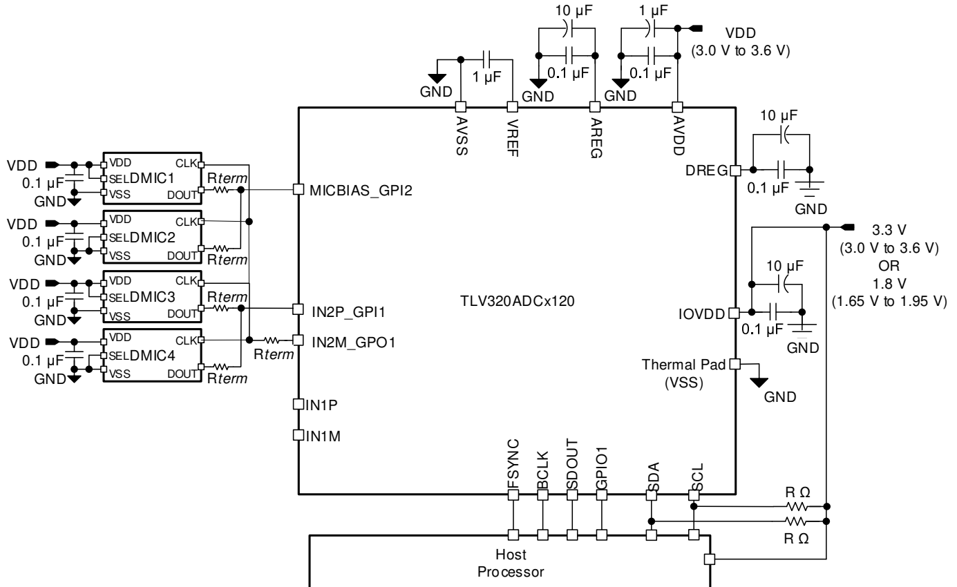
图 9-4. Four-Channel Digital PDM Microphone Recording Diagram
