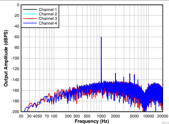
Figure 7-18. PDM Input FFT With a -60-dBr Input
