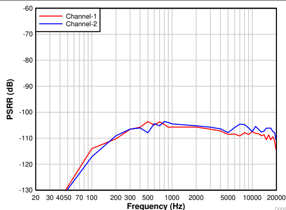
Figure 7-12. Power-Supply Rejection Ratio vs Ripple Frequency With 100-mV pp Amplitude
