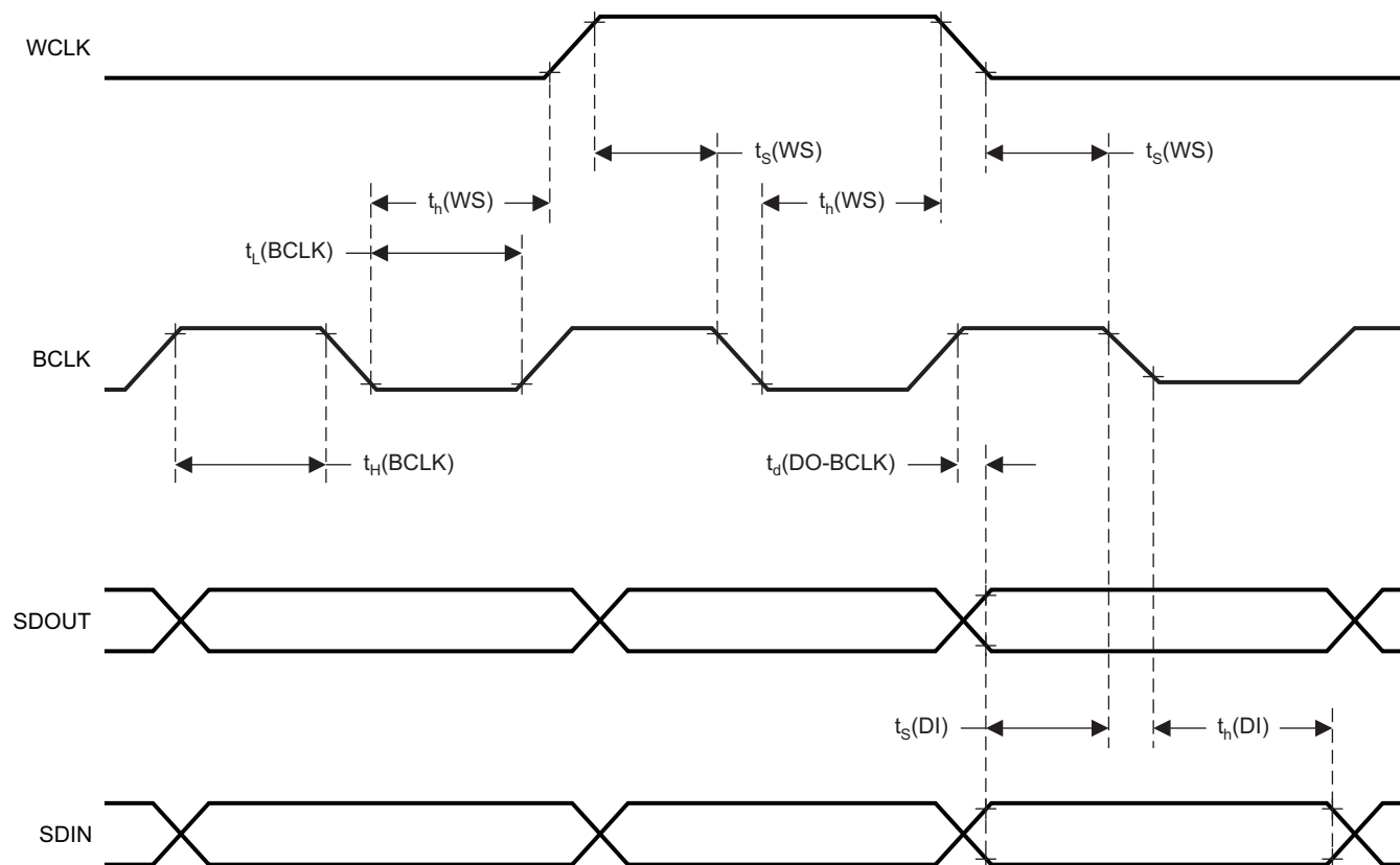
图 4. DSP Timing in Slave Mode
