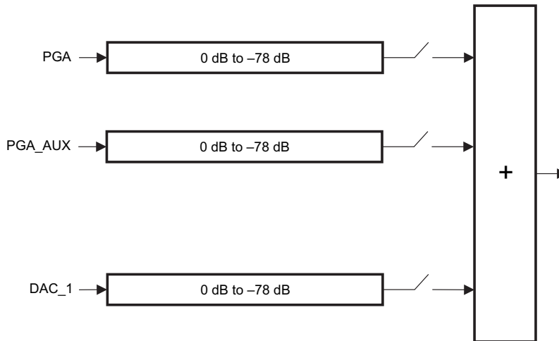
FIG 22. Detail of the Volume Control and Mixing Function in FIG 19 and FIG 29
