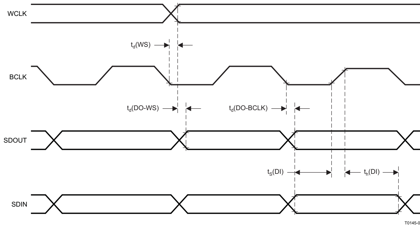
图 1. I²S, Left-Justified and Right-Justified Format Timing in Master Mode
