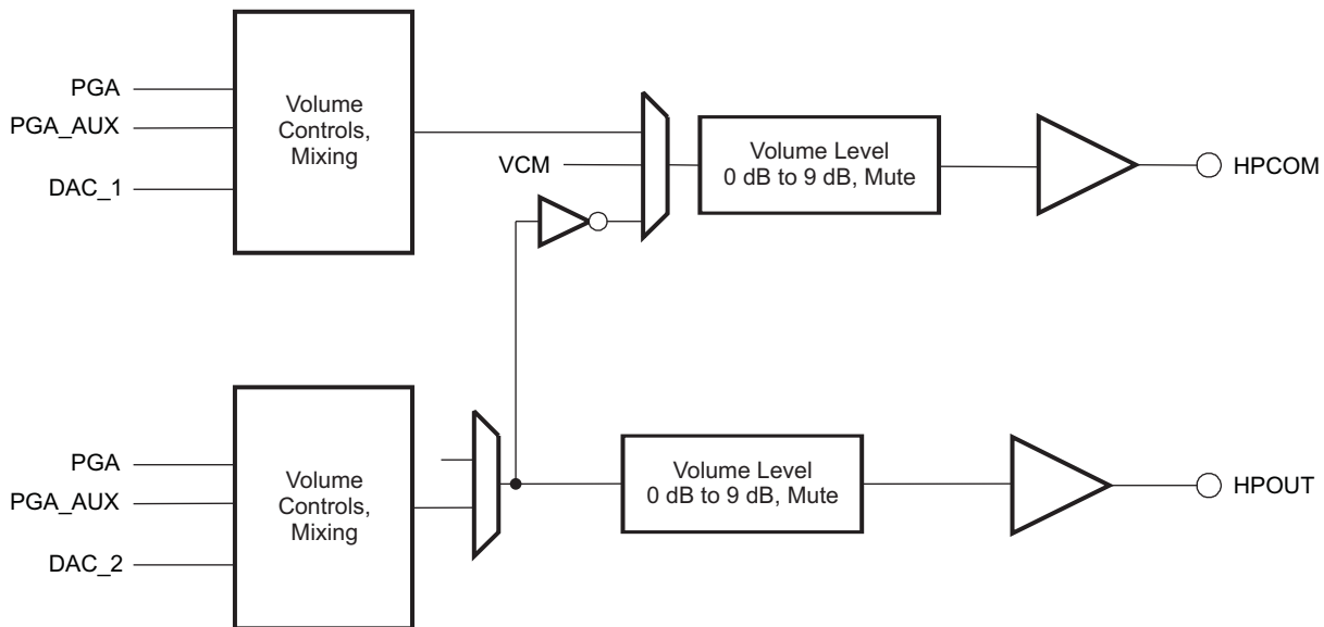
FIG 23. Architecture of the Output Stage Leading to the High-Power Output Drivers
