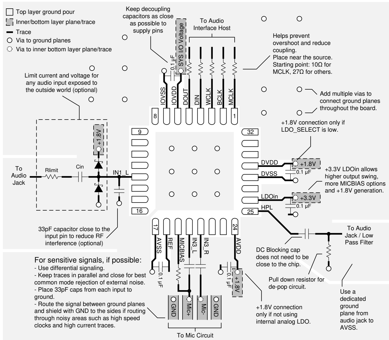
FIG 26. TLV320AIC3204 Layout
