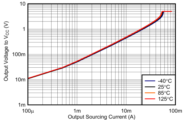
6-29. Output Voltage vs. Output Sourcing Current, 5 V
