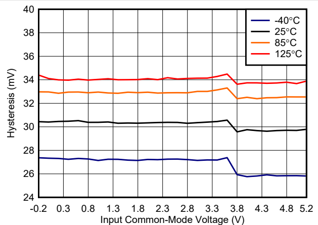
FIG 6-18. TLV3603 Hysteresis vs. Common-Mode, 5 V
