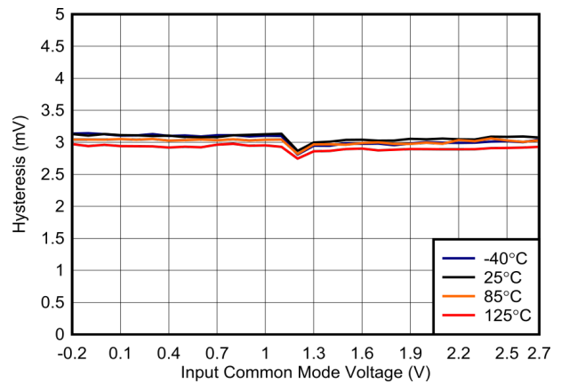
FIG 6-6. TLV3601 Hysteresis vs. Common-Mode, 2.5 V
