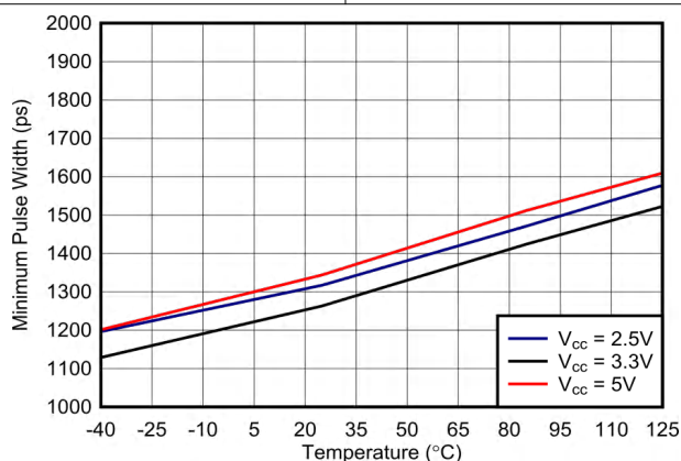
FIG 6-47. Minimum Pulse Width vs. Temperature
