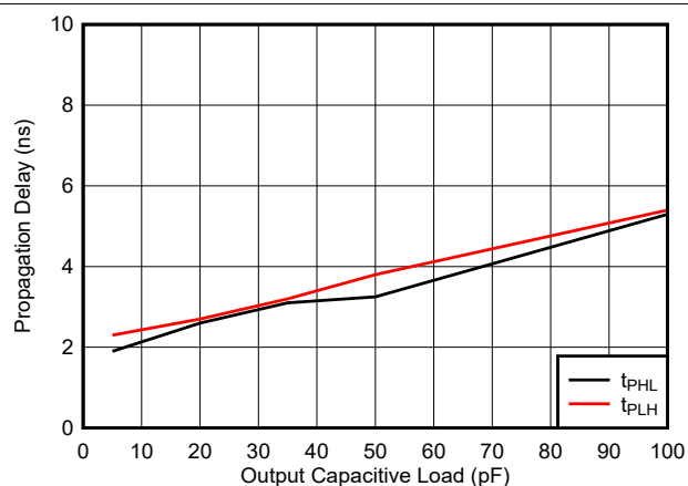
FIG 6-46. Propagation Delay vs. Load Capacitance, 5 V
