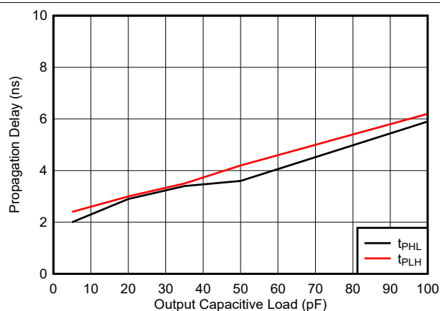
FIG 6-45. Propagation Delay vs. Load Capacitance, 3.3 V
