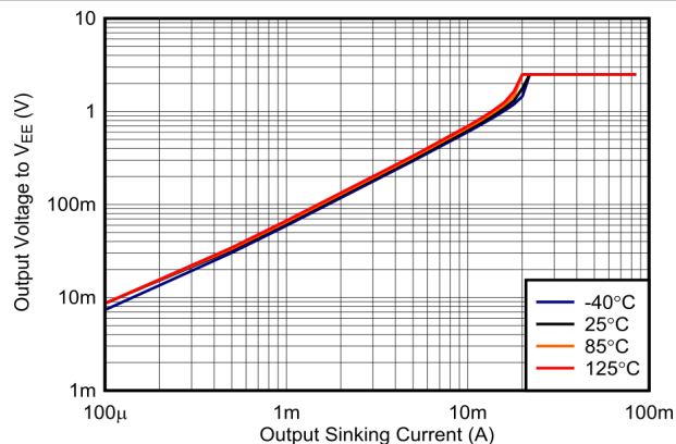
FIG 6-26. Output Voltage vs. Output Sinking Current, 2.5 V
