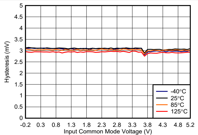
FIG 6-10. TLV3601 Hysteresis vs. Common-Mode, 5 V
