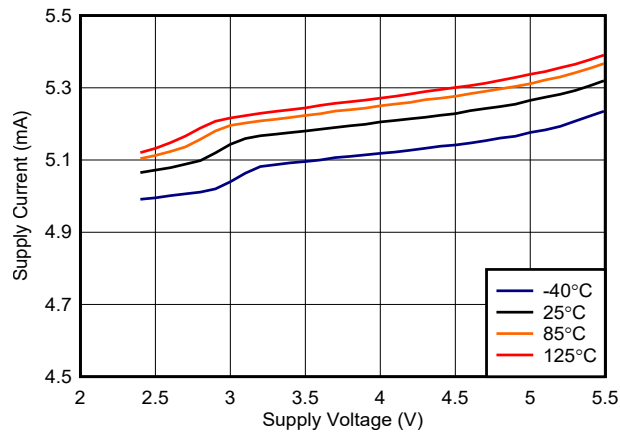
6-31. TLV3601 Supply Current vs. Voltage (Output Low)
