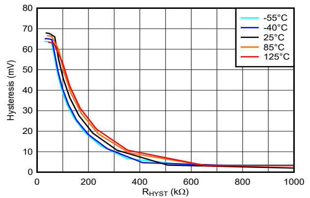
FIG 5-12. Hysteresis vs. Resistance, 3.3V
