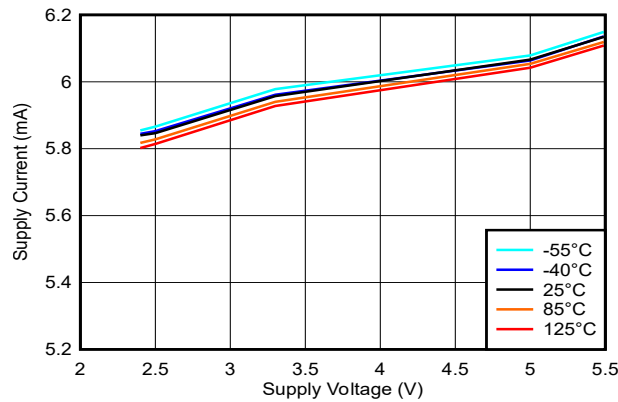
FIG 5-23. Supply Current vs. Voltage (Output Low)
