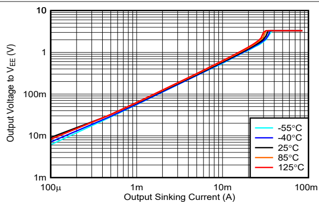
FIG 5-20. Output Voltage vs. Output Sinking Current, 3.3V
