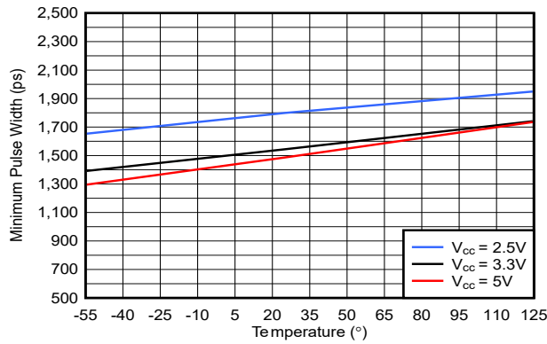
FIG 5-35. Minimum Pulse Width vs. Temperature
