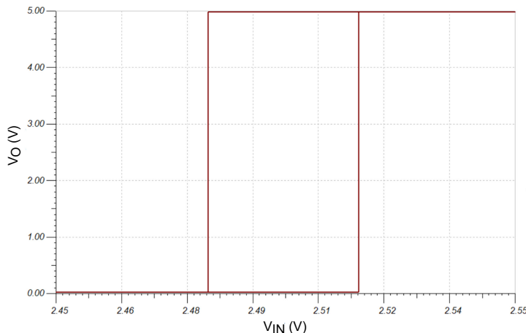
図 7-9. Hysteresis Transfer Curve using TLV3603-EP
