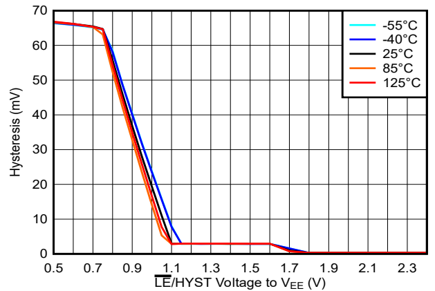
FIG 5-36. Hysteresis Voltage vs. \overline{\text{LE}}/\text{HYST} Voltage, 2.5V
