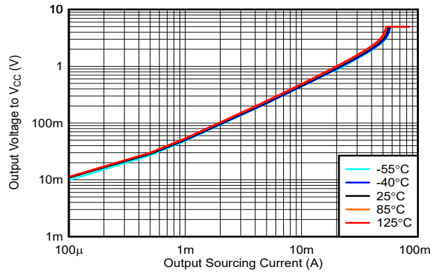
FIG 5-21. Output Voltage vs. Output Sourcing Current, 5V
