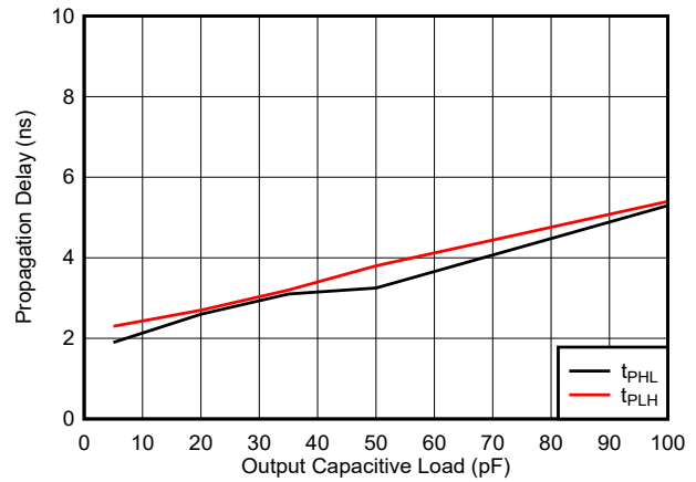
FIG 5-34. Propagation Delay vs. Load Capacitance, 5V
