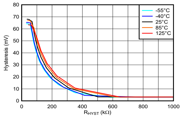
FIG 5-11. Hysteresis vs. Resistance, 2.5V
