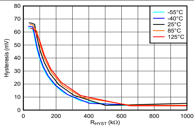
FIG 5-13. Hysteresis vs. Resistance, 5V
