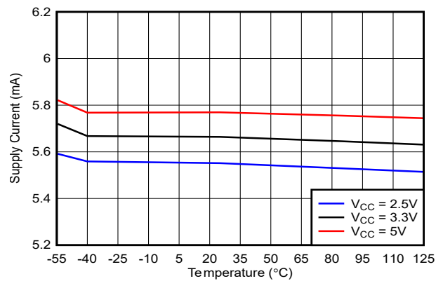
FIG 5-26. Supply Current vs. Temp (Output High)
