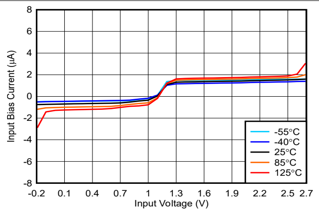
FIG 5-14. Bias Current vs. Input Voltage, 2.5V
