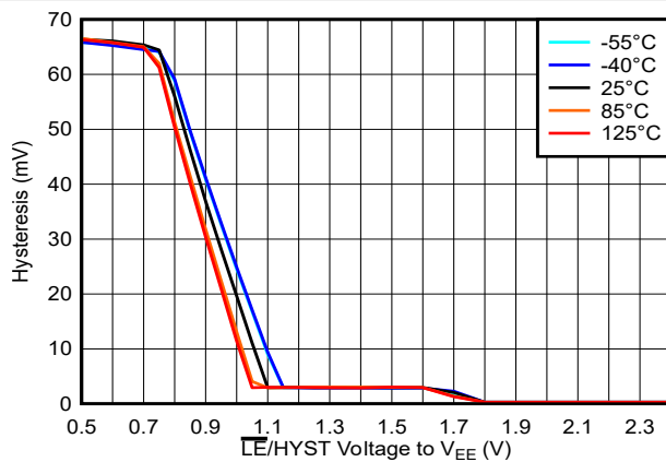
FIG 5-37. Hysteresis Voltage vs. \overline{\text{LE}}/\text{HYST} Voltage, 3.3V
