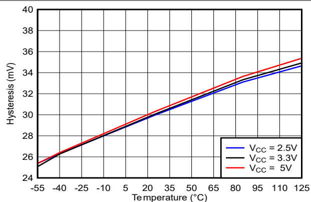
图 5-4. Hysteresis vs. Temperature
