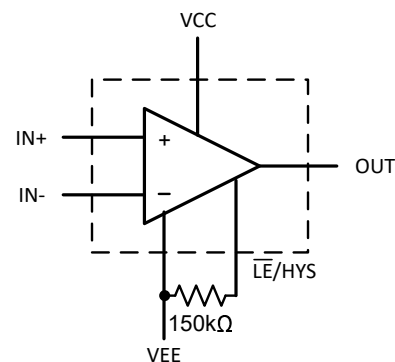
図 7-8. Setting the Hysteresis using a Resistor using the TLV3603-EP
