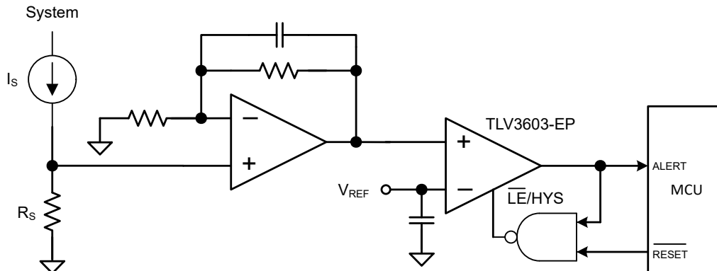
図 7-11. Over-Current Latched Output Circuit
