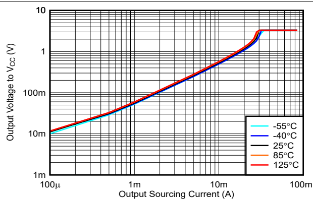
FIG 5-19. Output Voltage vs. Output Sourcing Current, 3.3V
