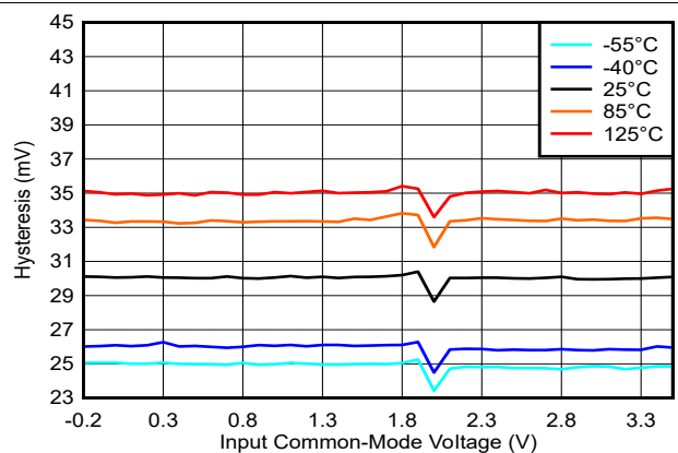
图 5-8. Hysteresis vs. Common-Mode, 3.3V
