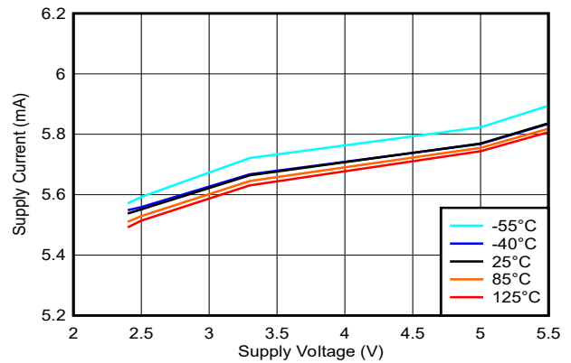
FIG 5-24. Supply Current vs. Voltage (Output High)
