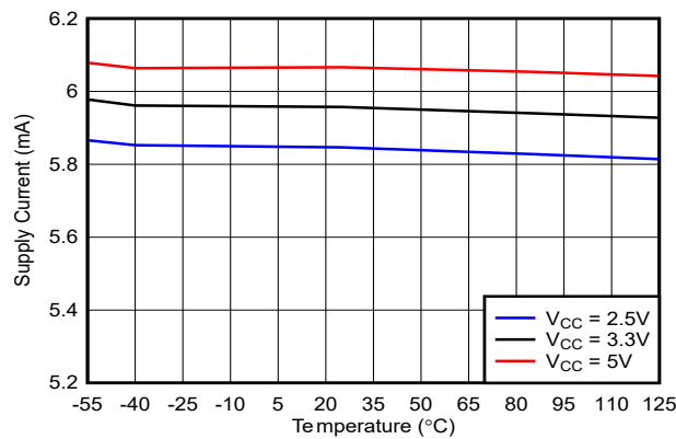
FIG 5-25. Supply Current vs. Temp (Output Low)
