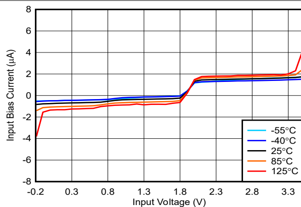
FIG 5-15. Bias Current vs. Input Voltage, 3.3V
