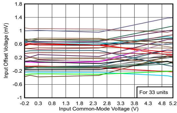
FIG 5-9. Offset vs. Common-Mode, 5V
