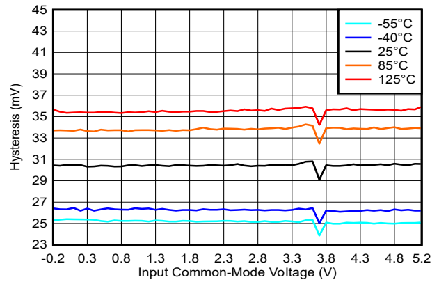
FIG 5-10. Hysteresis vs. Common-Mode, 5V
