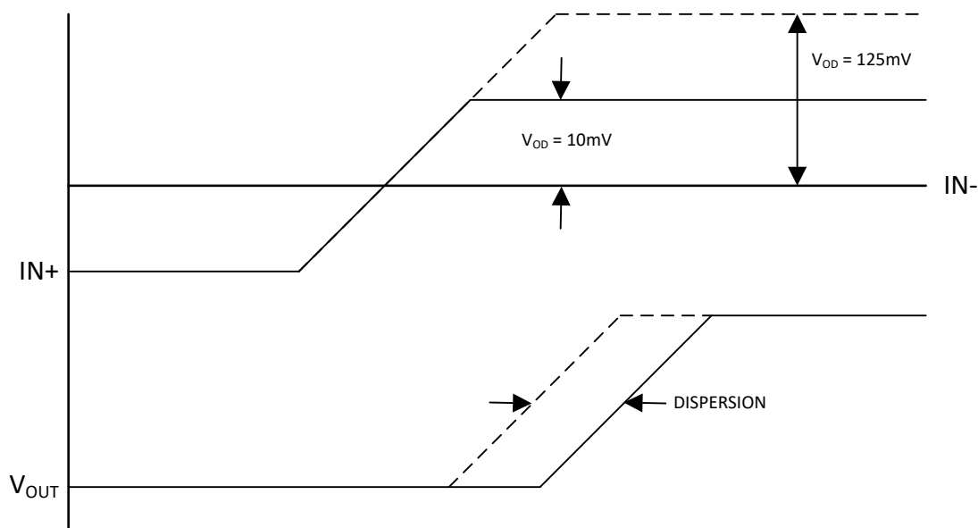
図 5-2. Overdrive Dispersion
