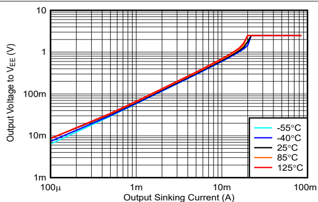
FIG 5-18. Output Voltage vs. Output Sinking Current, 2.5V
