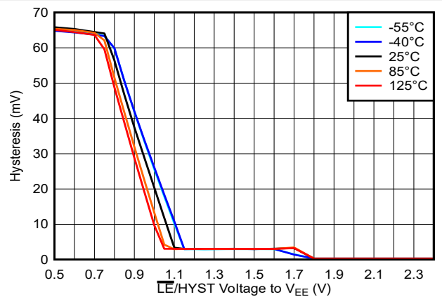
FIG 5-38. Hysteresis Voltage vs. \overline{\text{LE}}/\text{HYST} Voltage, 5V
