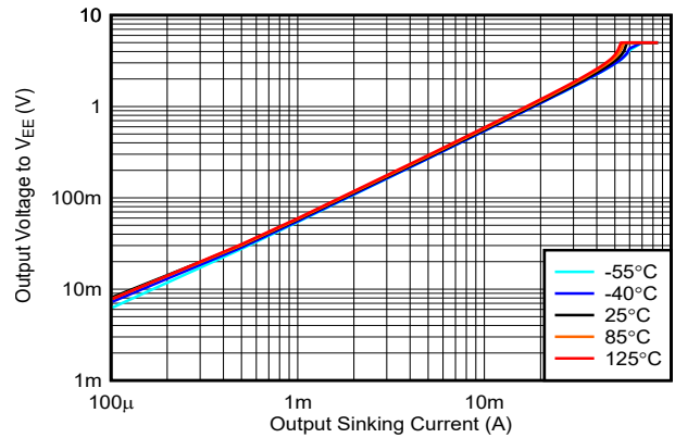
FIG 5-22. Output Voltage vs. Output Sinking Current, 5V
