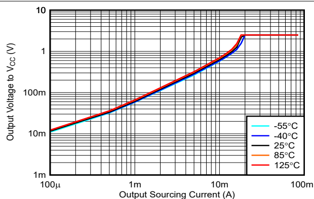
FIG 5-17. Output Voltage vs. Output Sourcing Current, 2.5V
