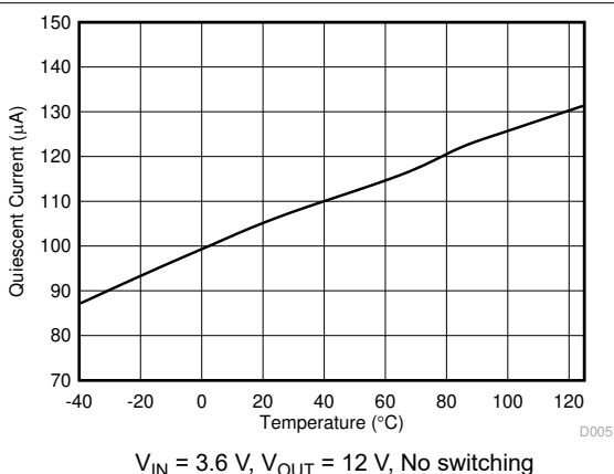
Figure 6-5. Quiescent Current into VIN vs Temperature
