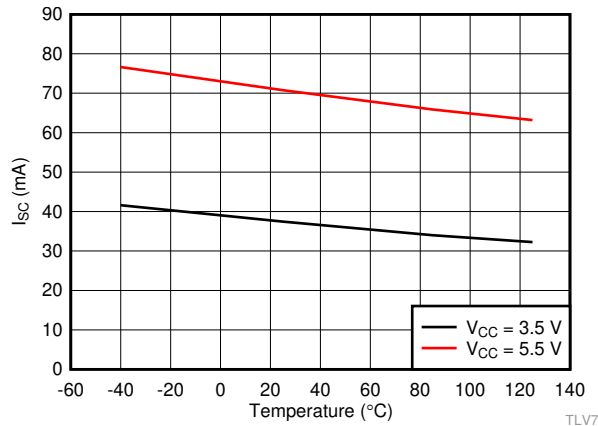
图 27. TLV7011 Output Short-Circuit (Source) Current vs. Temperature
