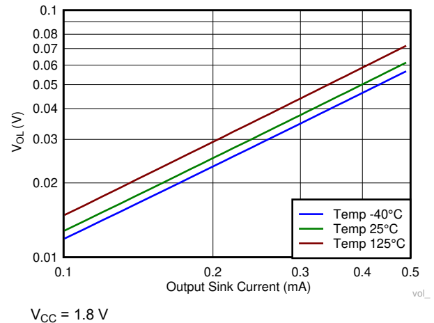
6-16. Output Voltage Low vs Output Sink Current
