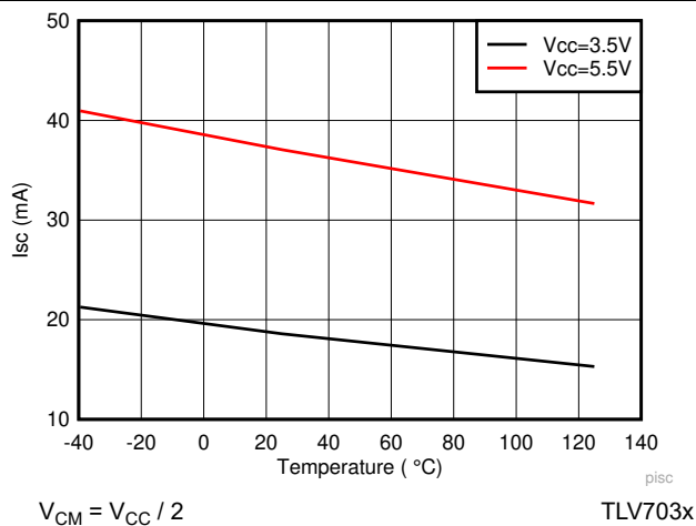
6-19. Output Short-Circuit (Source) Current vs Temperature
