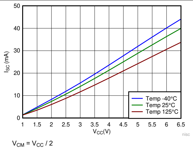
6-20. Output Short Circuit (Sink) vs V_{CC}
