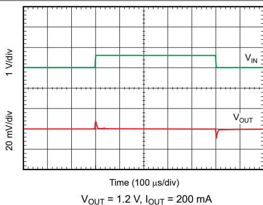
6-47. Line Transient Response
