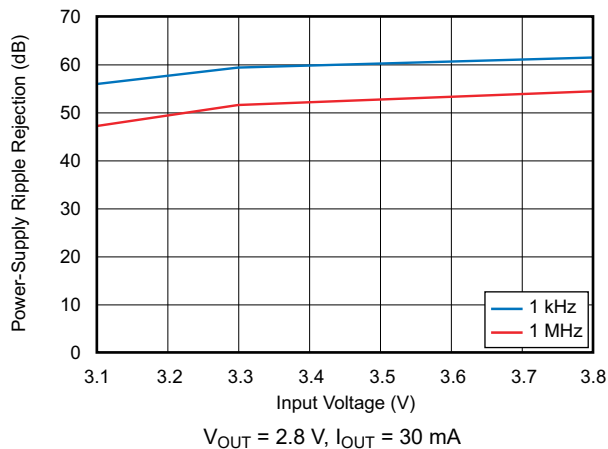
FIG 6-35. Power-Supply Ripple Rejection vs Input Voltage
