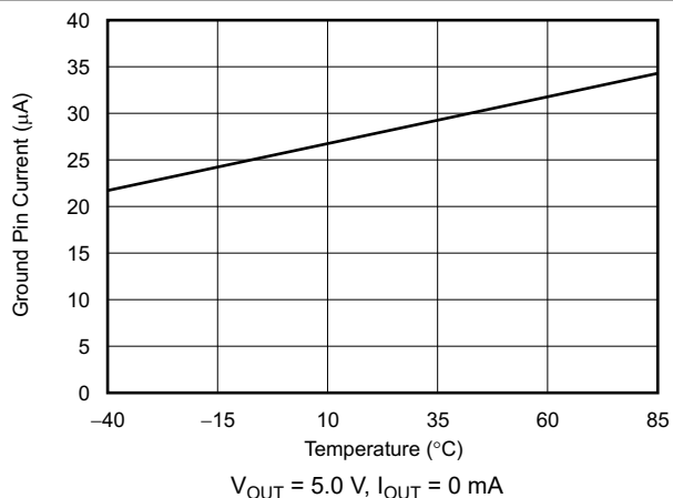
FIG 6-22. Ground Pin Current vs Temperature
