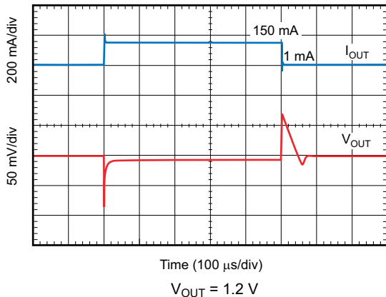
8-4. Load Transient Response
