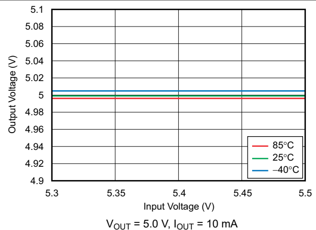
Figure 6-6. Line Regulation
