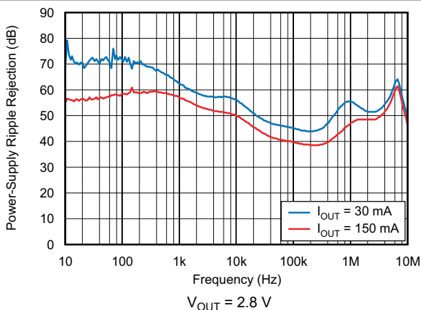
FIG 6-33. Power-Supply Ripple Rejection vs Frequency
