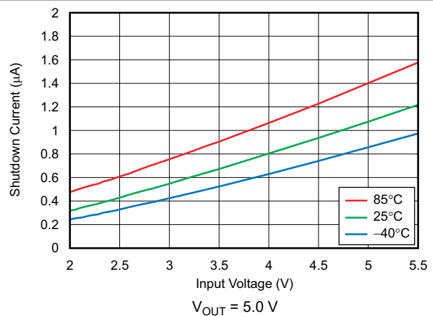
6-28. Shutdown Current vs Input Voltage
