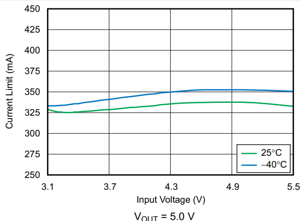
FIG 6-31. Current Limit vs Input Voltage
