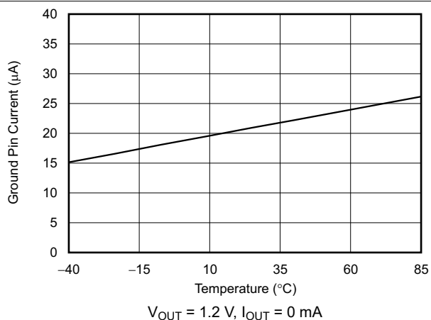
FIG 6-20. Ground Pin Current vs Temperature
