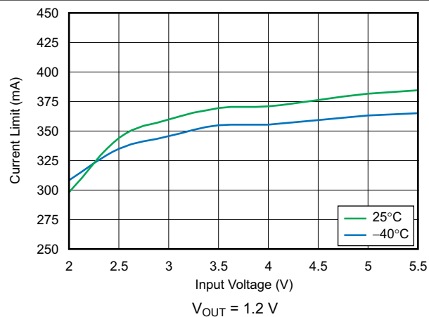
6-29. Current Limit vs Input Voltage
