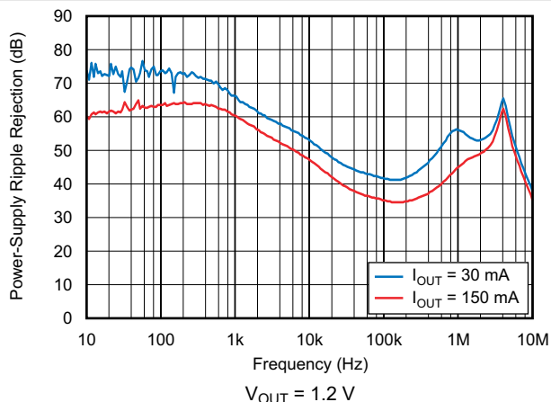
FIG 6-32. Power-Supply Ripple Rejection vs Frequency
