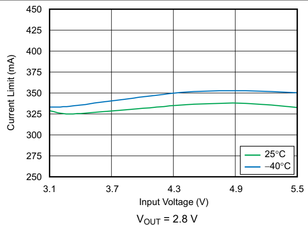
6-30. Current Limit vs Input Voltage
