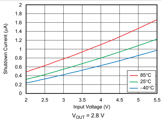
6-27. Shutdown Current vs Input Voltage
