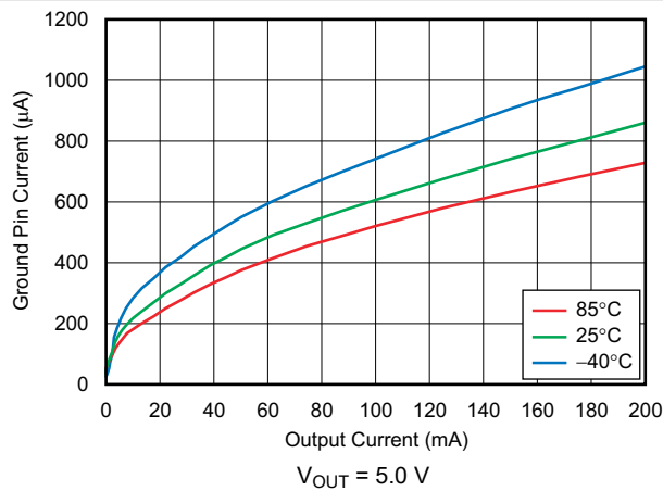
6-25. Ground Pin Current vs Output Current
