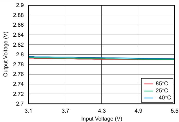
Figure 6-8. Line Regulation
