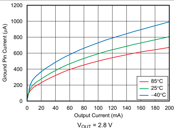
FIG 6-24. Ground Pin Current vs Output Current
