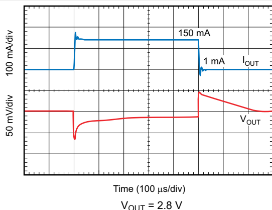
6-43. Load Transient Response
