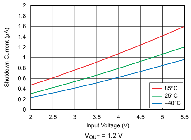
6-26. Shutdown Current vs Input Voltage
