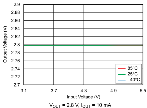
Figure 6-5. Line Regulation
