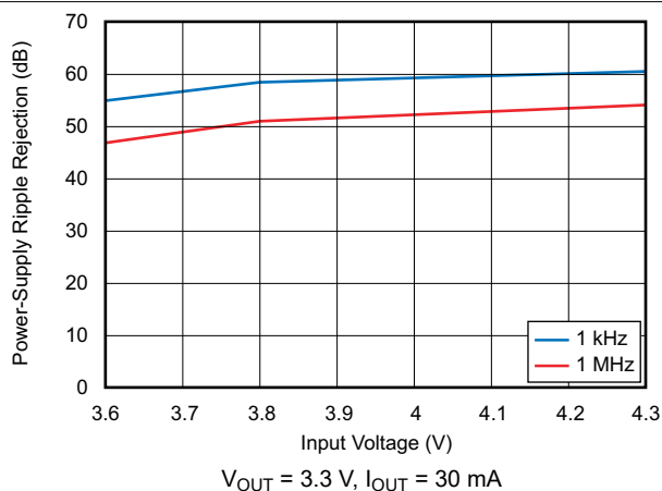
FIG 6-37. Power-Supply Ripple Rejection vs Input Voltage
