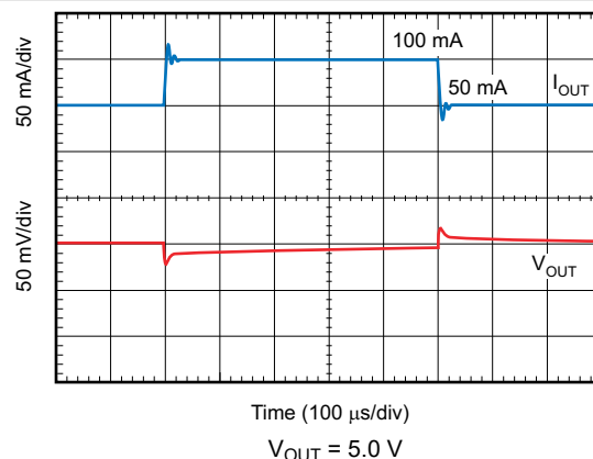
6-44. Load Transient Response
