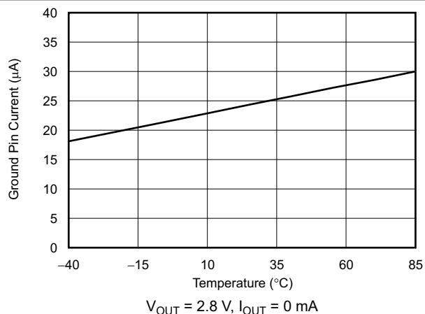
FIG 6-21. Ground Pin Current vs Temperature
