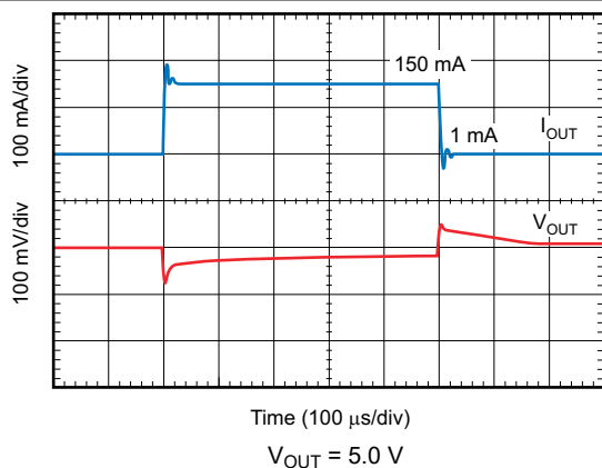
6-45. Load Transient Response
