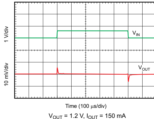
8-5. Line Transient Response
