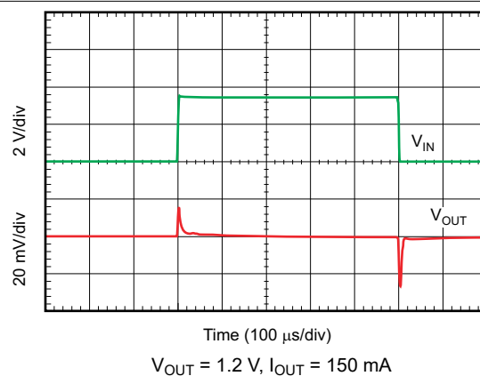
6-48. Line Transient Response
