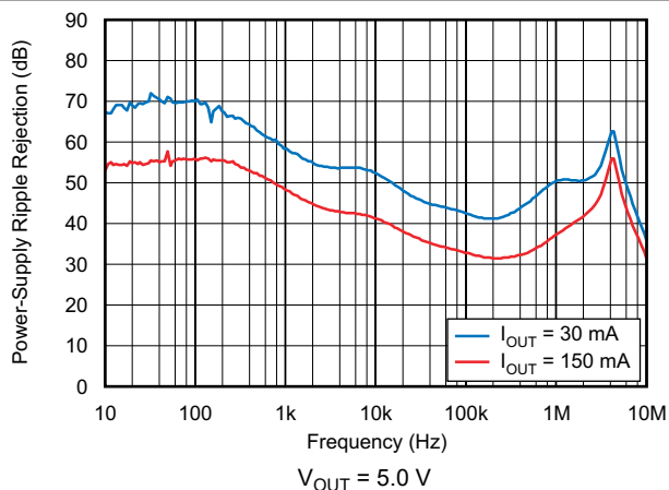
FIG 6-34. Power-Supply Ripple Rejection vs Frequency
