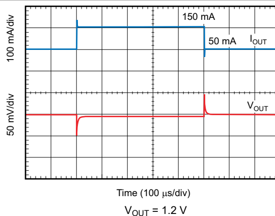
FIG 6-40. Load Transient Response
