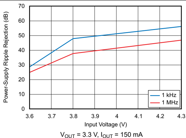
FIG 6-38. Power-Supply Ripple Rejection vs Input Voltage
