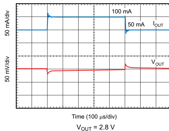
FIG 6-42. Load Transient Response
