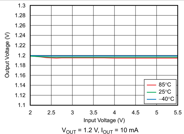
Figure 6-4. Line Regulation
