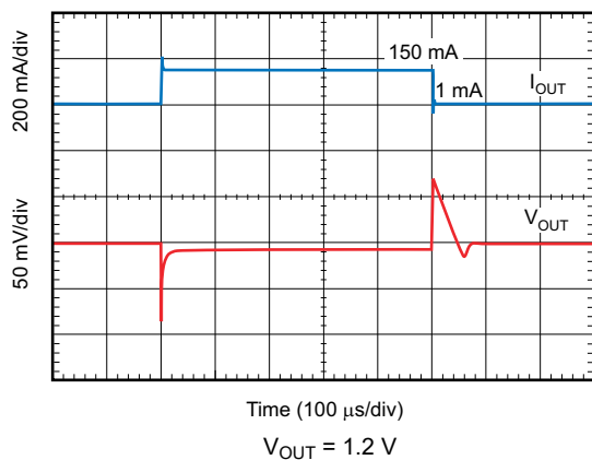
FIG 6-41. Load Transient Response
