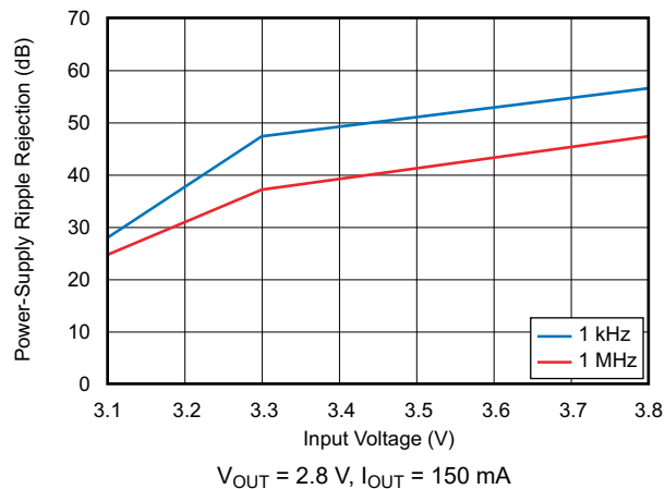
FIG 6-36. Power-Supply Ripple Rejection vs Input Voltage
