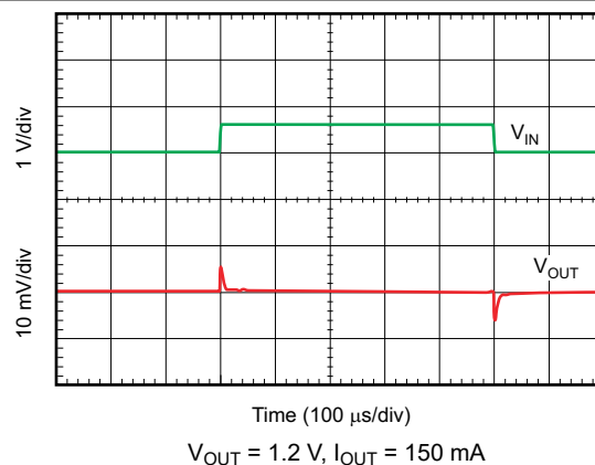
6-46. Line Transient Response
