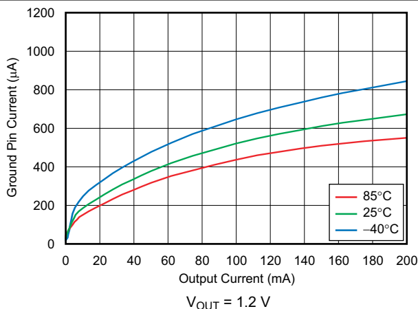
FIG 6-23. Ground Pin Current vs Output Current
