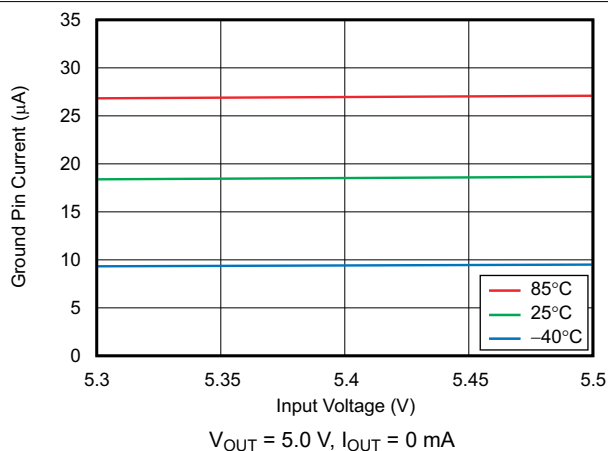
FIG 6-19. Ground Pin Current vs Input Voltage
