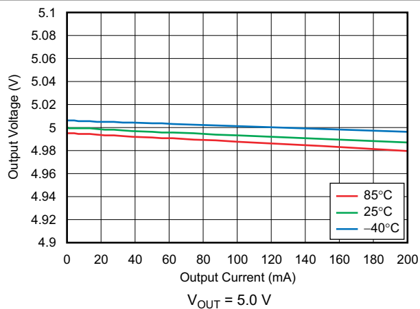
Figure 6-3. Load Regulation
