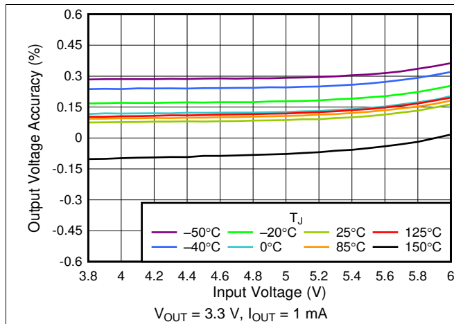
Fig. 1. 3.3-V Line Regulation vs V_{IN}
