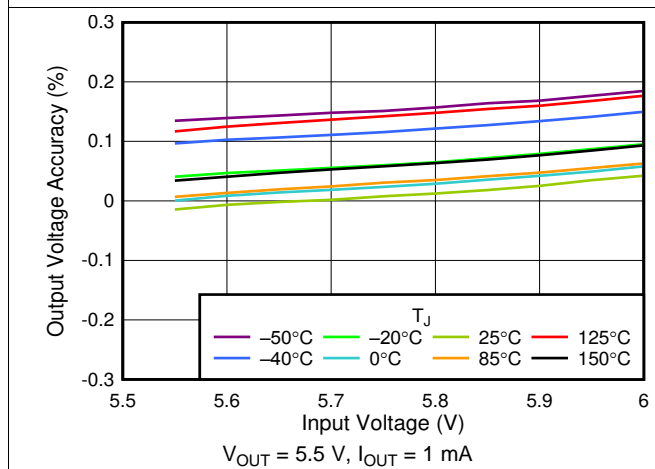
Fig. 3. 5.5-V Line Regulation vs V_{IN}
