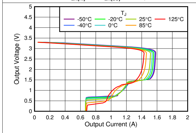
图 17. 3.3-V Foldback Current Limit vs I_{OUT}
