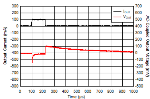
図 7-3. I_{OUT} Transient From 0 mA to 100 mA
