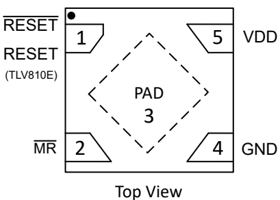
6-5. DPW Package 5-Pin X2SON See 表 6-1 Top View
