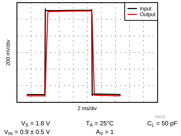
Figure 28. Large Signal Pulse Response, 1.8 V
