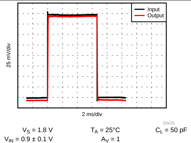
Figure 26. Small Signal Pulse Response, 1.8 V
