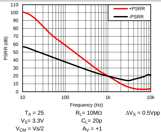
Figure 24. \pm\text{PSRR} vs Frequency
