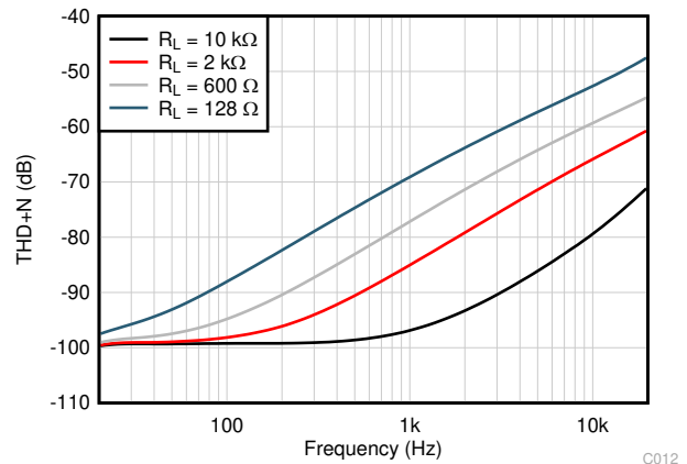
6-20. THD+N Ratio vs Frequency
